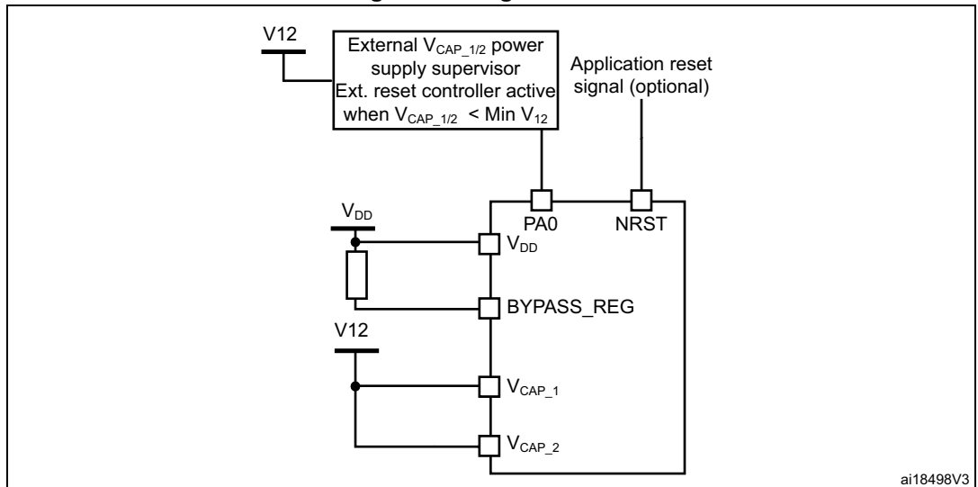
Figure 12. Regulator OFF
