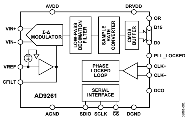
Figure 1. AD9261 Functional Block Diagram
