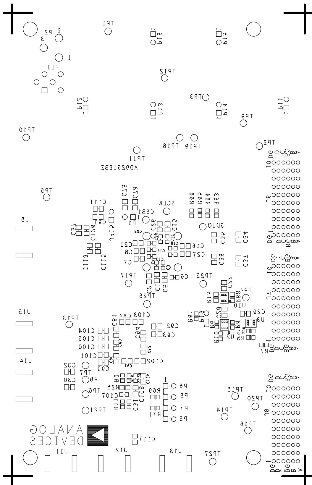
Figure 19. Bottom Silk
