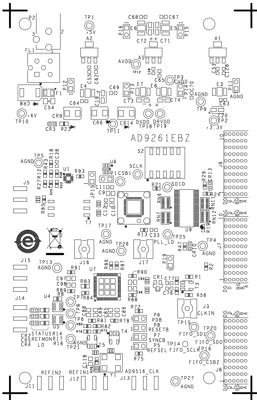
Figure 18. Top Silk
