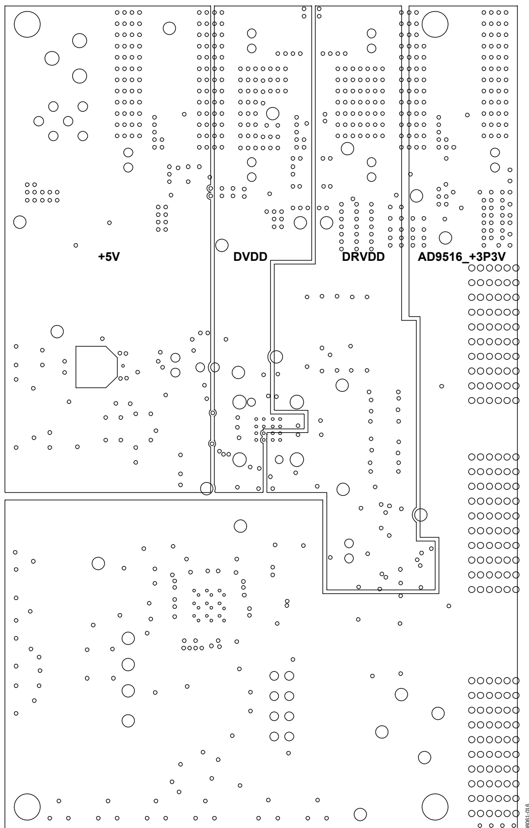
Figure 21. Power Layer 4
