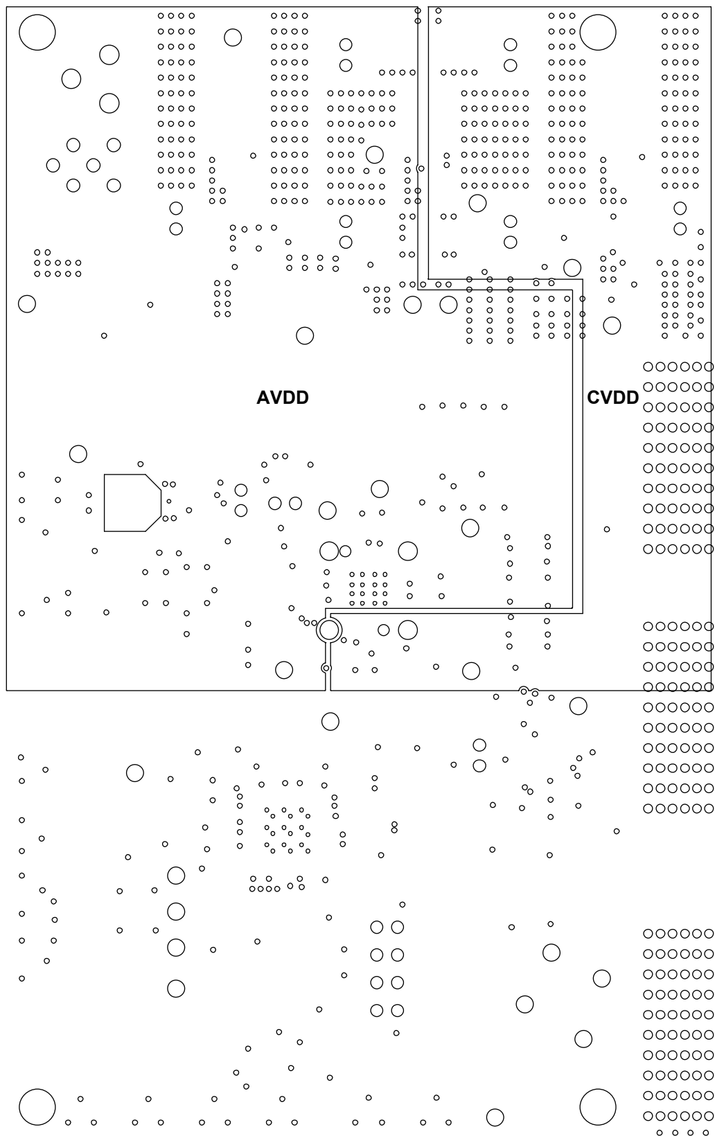
Figure 20. Power Layer 3
