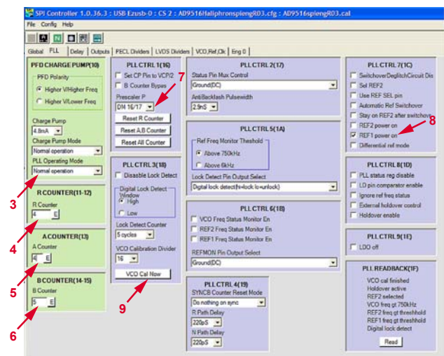
Figure 11. PLL Configuration for the 122.88 MHz Crystal Oscillator
