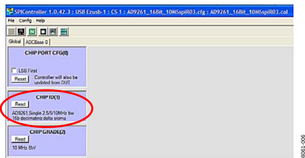
Figure 6. AD9261 SPIController
