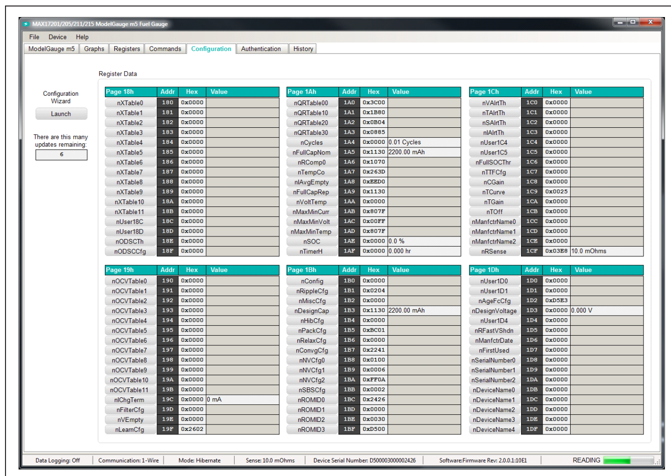
Figure 9. Configuration Tab
