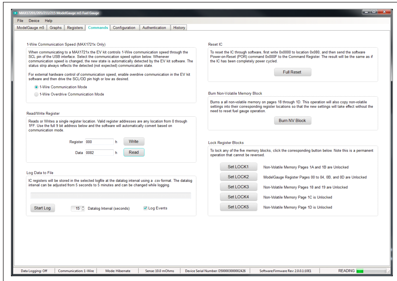
Figure 8. Commands Tab
