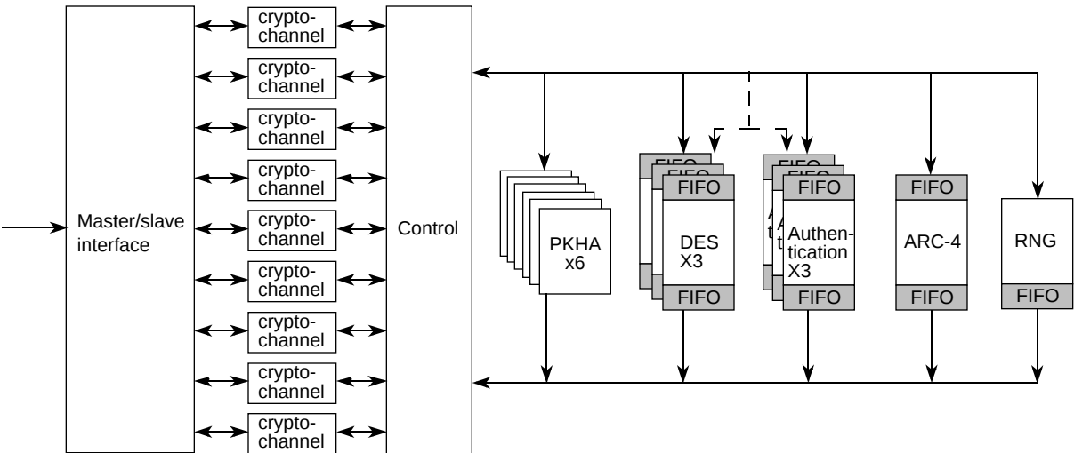
Figure 5-3. MPC190 Block Diagram
