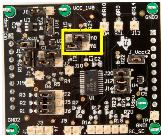
Figure 5. A0 and A1 Slave Address Configuration
