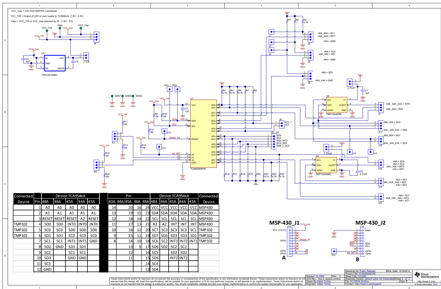
Figure 13. TCA9548AEVM Schematic
