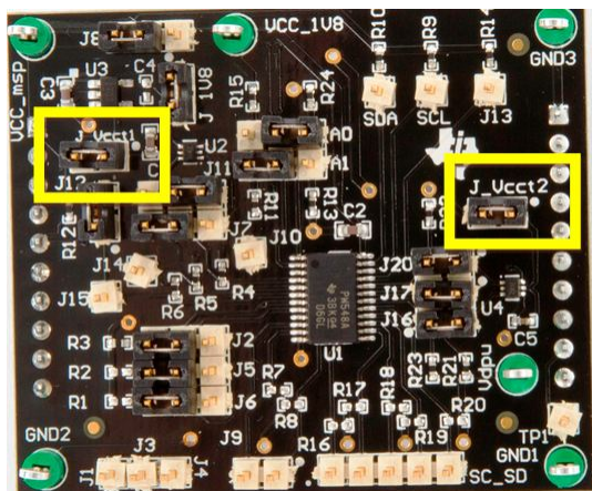
Figure 4. J_Vcct1 and J_Vcct2 Jumper Connections
