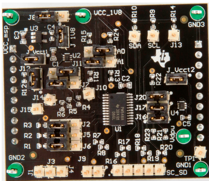
Figure 1. TCA9548AEVM
