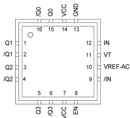
16-Pin 3mm × 3mm QFN
