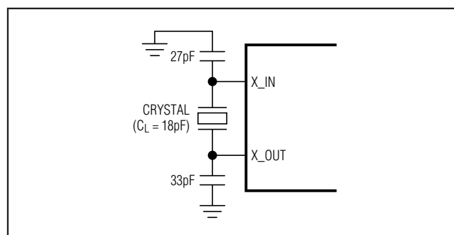
Figure 7. Crystal, Capacitors Connection
