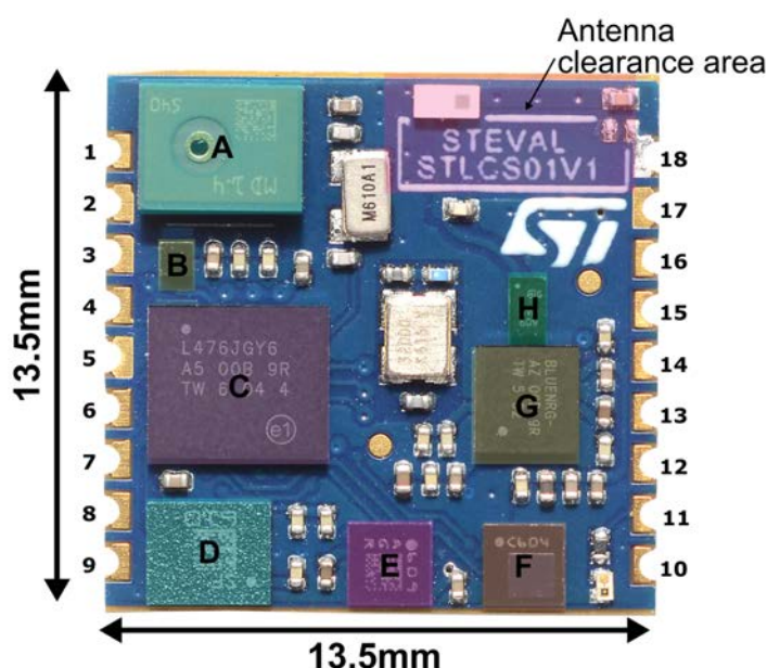
Figure 5. STEVAL-STLCS01V1 main components and pinout
