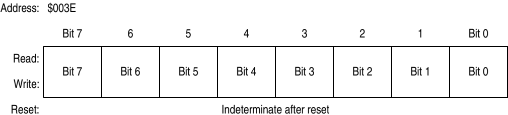
Figure 3-5. ADC Data Register (ADR)
