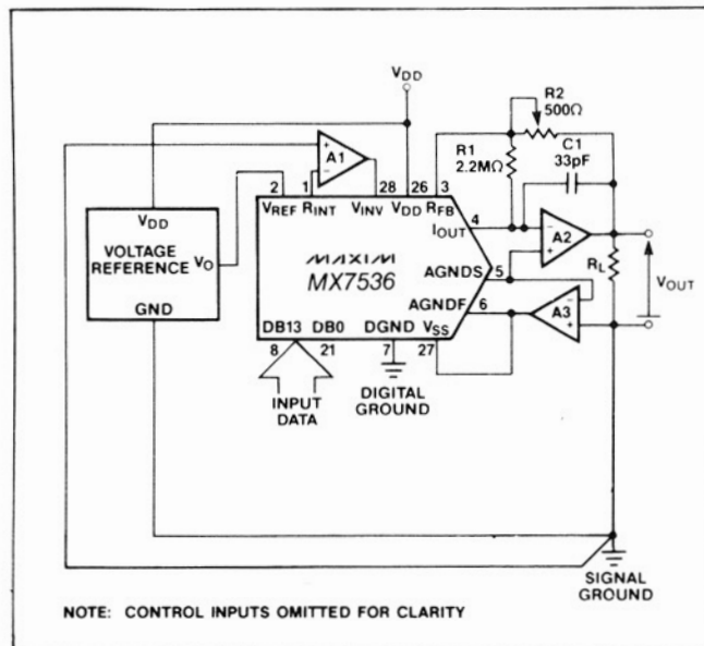
Figure 5. MX7536 Operation with Forced Ground
