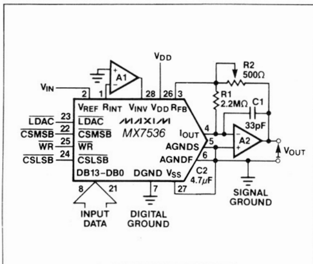
Figure 4. MX7536 Operation
