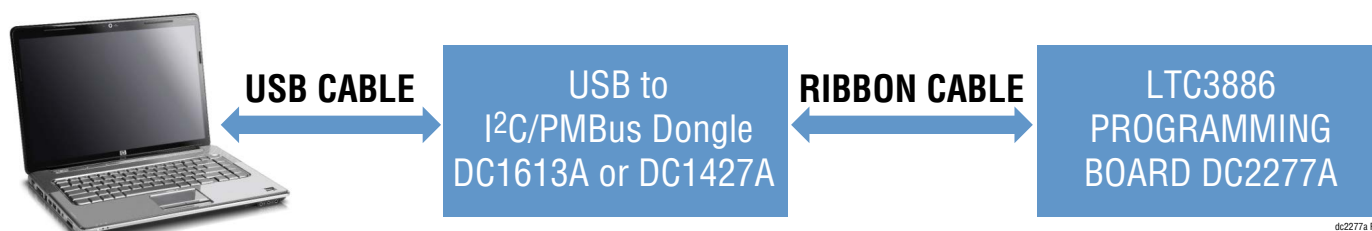
Figure 1. LTC3886 Programming Setup Using the DC2277A
