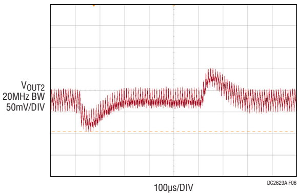
Figure 6. DC2529A V_{OUT2} 1.25A to 2.5A Load Transient at V_{IN} = 48V
