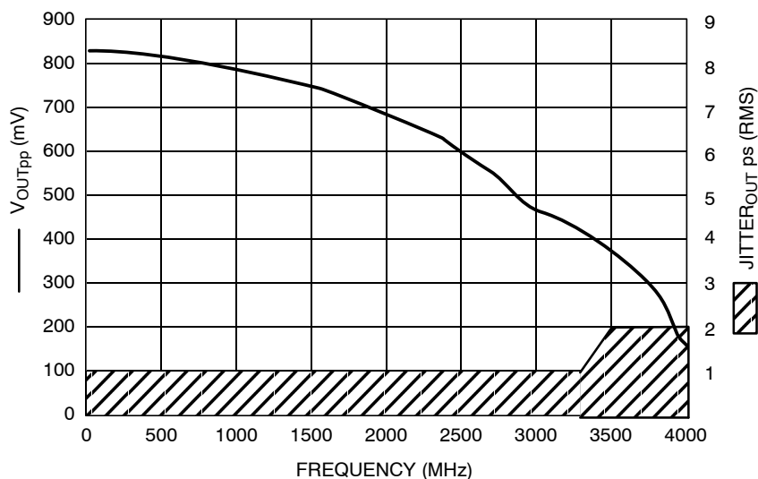
Figure 2. F_{\max} /Jitter for QH\bar{G} , \bar{QH}\bar{G} Output
