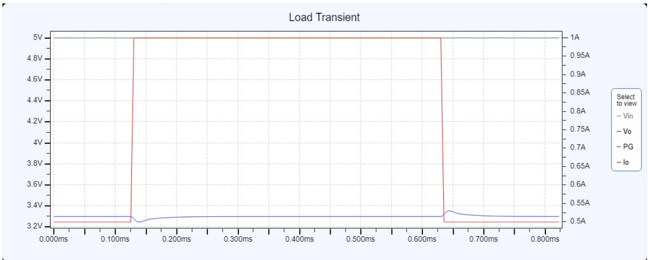
Vin = 6V, Ihigh = 1A, Ilow = 0.5A, Slew rate = 0.1A/μs
