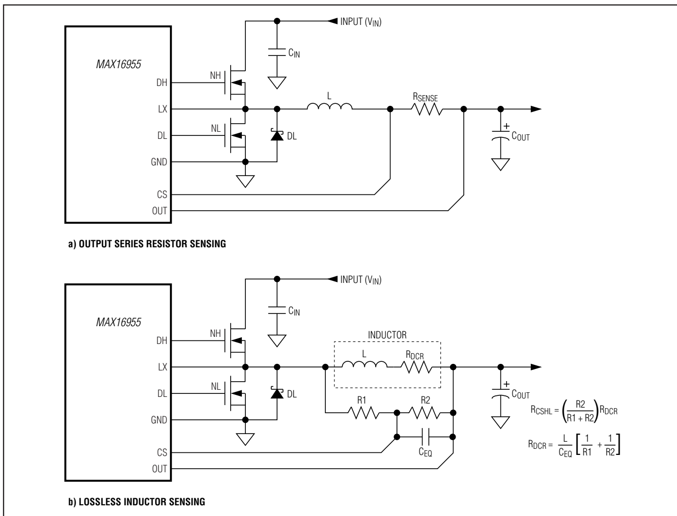
Figure 4. Current-Sense Configurations
