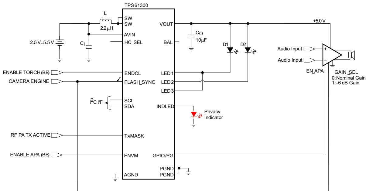
Figure 102. White LED Flashlight Driver and Audio Amplifier Power Supply Exclusive Operation
