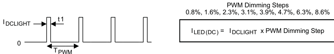
Figure 41. PWM Dimming Principle
