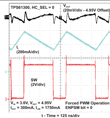
Figure 93. PWM Operation
