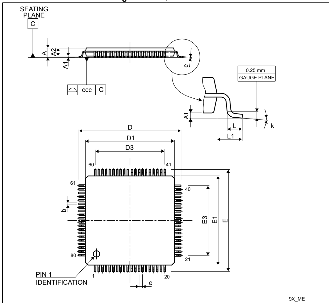
Figure 65. LQFP80 - outline
