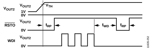
Figure 52. Watchdog Timing Diagram
