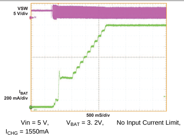
Figure 4. Charge Current Ramp Up
