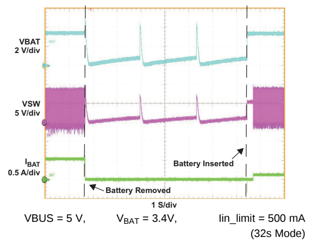
Figure 29. Battery Insertion/Removal
