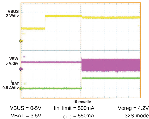
Figure 28. Adapter Insertion
