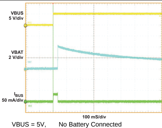
Figure 28. Adapter Insertion
