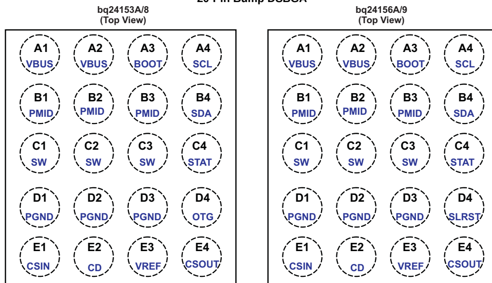
YFF Package 20-Pin Bump DSBGA
