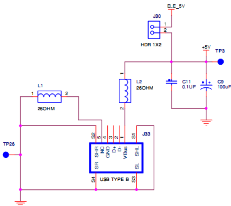
Figure 4. Power Inputs
