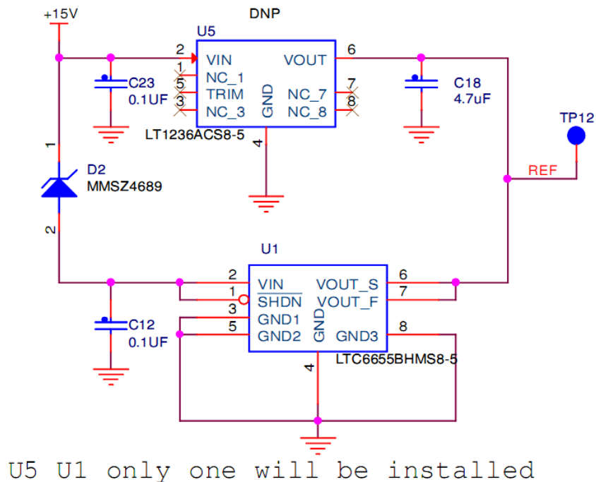
Figure 6. LTC6655-5 Voltage Reference
