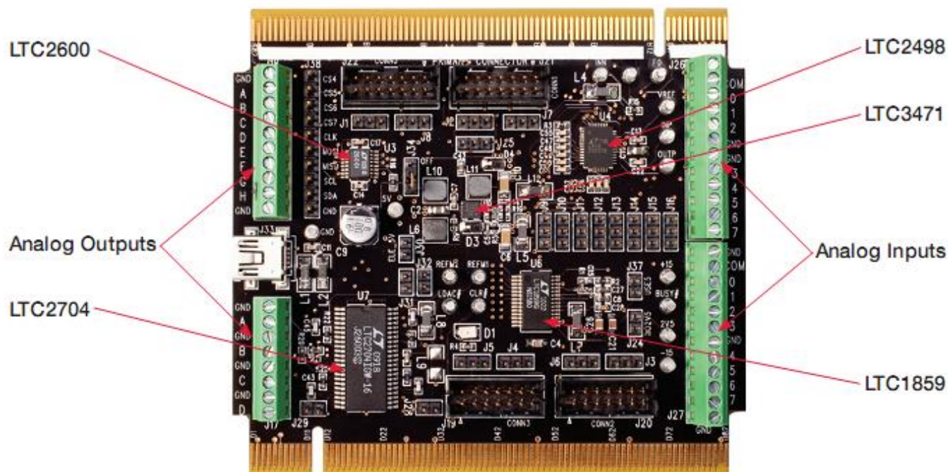
Figure 2. Callouts on top side of the TWR-ADCDAC-LTC
