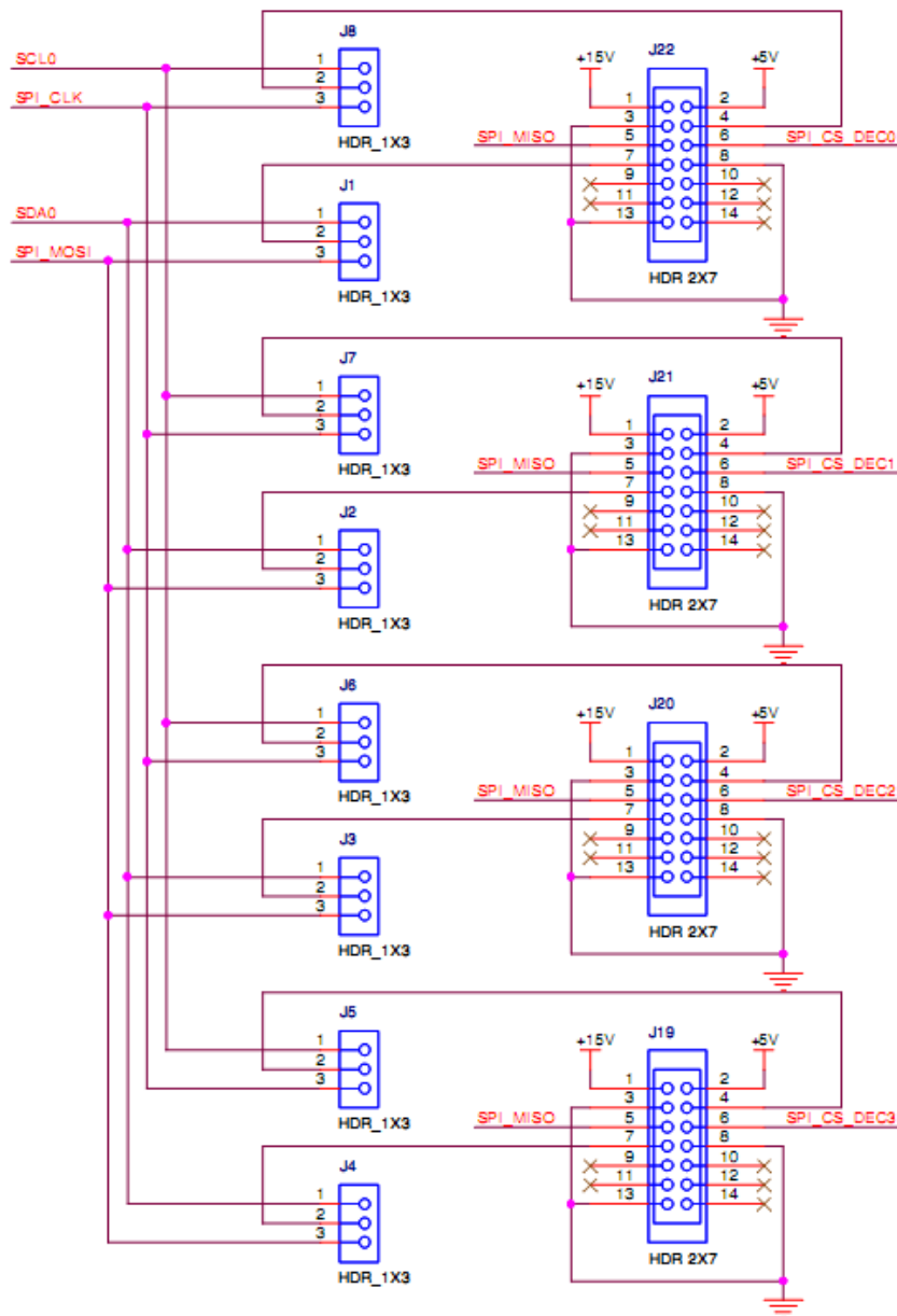
Figure 7. QuikEval Connectors
