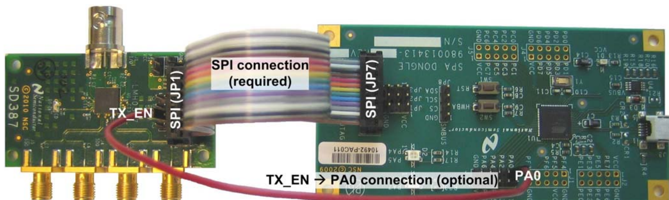
FIGURE 3. SD387 Connection to SPA Dongle
