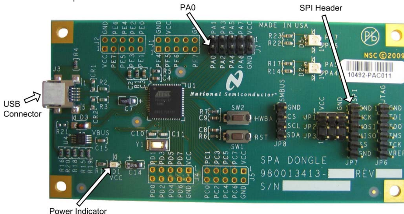
FIGURE 2. SPA Dongle
