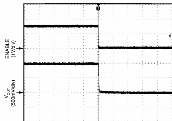
Turn-Off Transient
