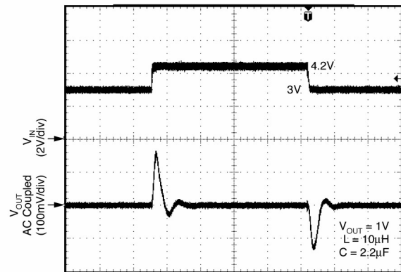
Line Transient
