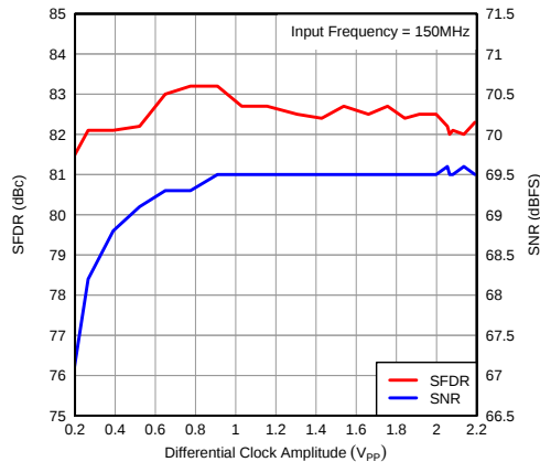
Figure 86. Performance vs Input Clock Amplitude
