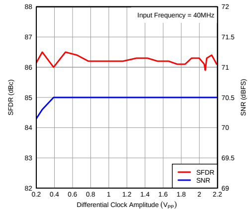
Figure 85. Performance vs Input Clock Amplitude
