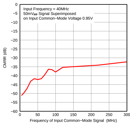
Figure 124. CMRR vs Test Signal Frequency
