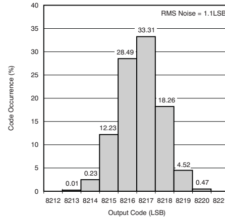
Figure 69. Output Noise Histogram (With Inputs Shorted to VCM)
