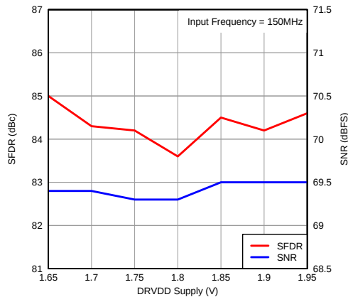
Figure 84. Performance vs DRVDD Supply Voltage
