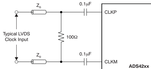
Figure 145. LVDS Clock Driving Circuit
