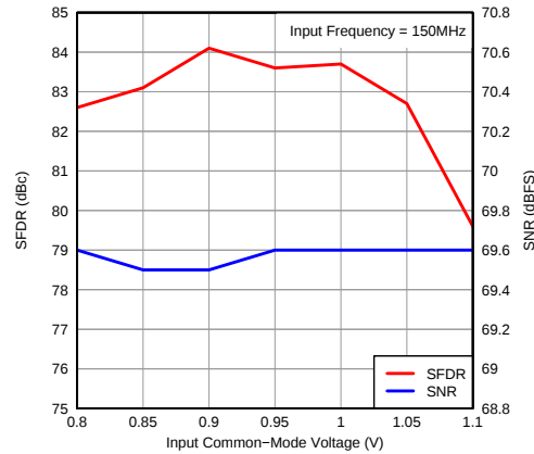
Figure 117. Performance vs Input Common-Mode Voltage
