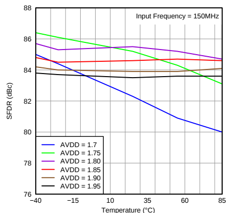
Figure 62. SFDR vs Temperature and AVDD Supply
