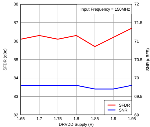
Figure 100. Performance vs DRVDD Supply Voltage
