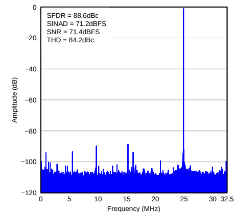
Figure 49. FFT for 170-MHz Input Signal
