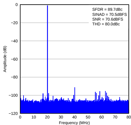
Figure 70. FFT for 20-MHz Input Signal
