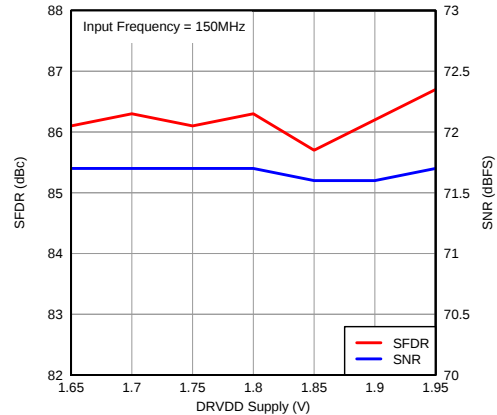
Figure 43. Performance vs DRVDD Supply Voltage
