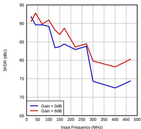
Figure 109. SFDR vs Input Frequency
