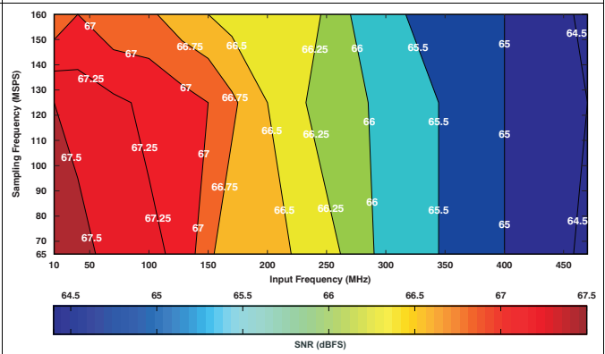
Figure 132. ADS424x Signal-to-Noise Ratio (6-dB Gain)
