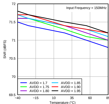
Figure 63. SNR vs Temperature and AVDD Supply
