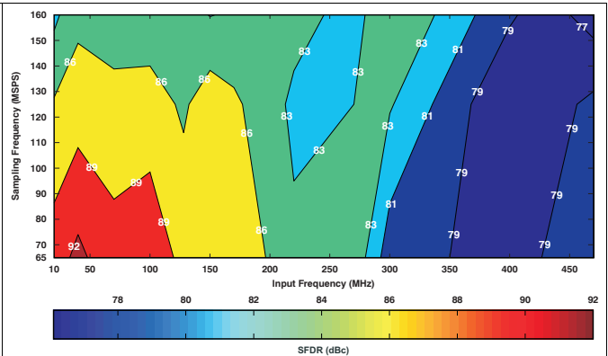
Figure 130. Spurious-Free Dynamic Range (6-dB Gain)
