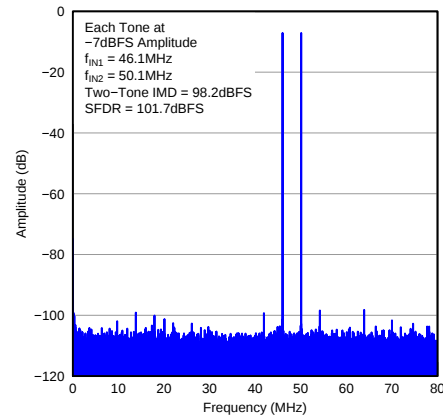
Figure 73. FFT for Two-Tone Input Signal
