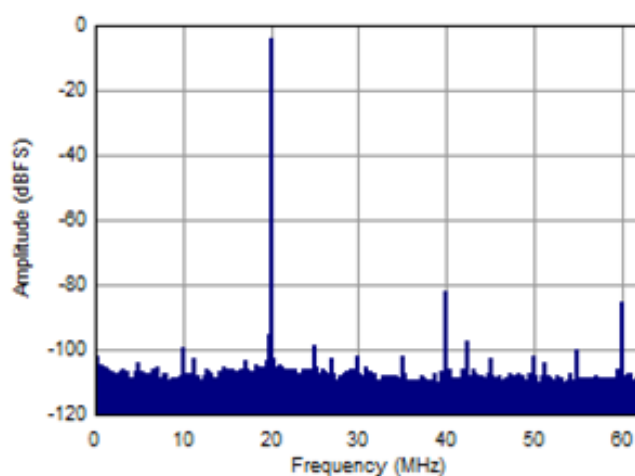
Figure 163. FFT for 270-MHz Input Signal
