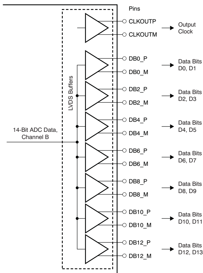
Figure 154. LVDS Interface
