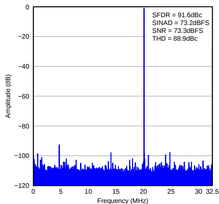
Figure 48. FFT for 20-MHz Input Signal
