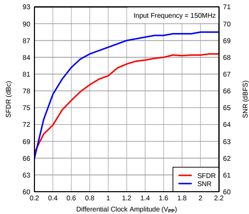
Figure 122. Performance vs Input Clock Amplitude
