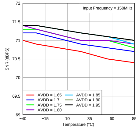
Figure 21. SNR vs Temperature and AVDD Supply
