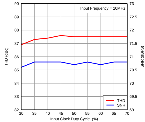
Figure 103. Performance vs Input Clock Duty Cycle
