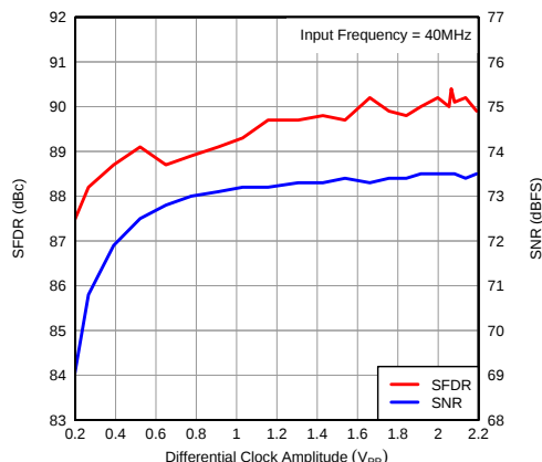
Figure 65. Performance vs Input Clock Amplitude
