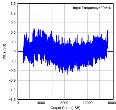
Figure 46. Integrated Nonlinearity
