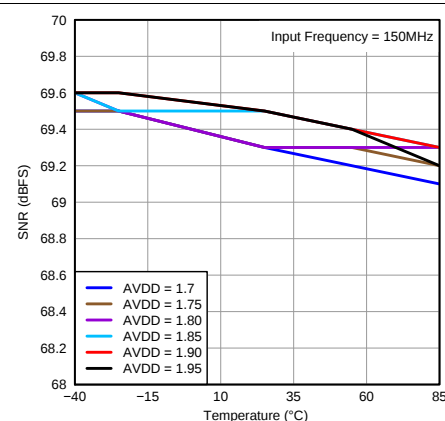
Figure 83. SNR vs Temperature and AVDD Supply
