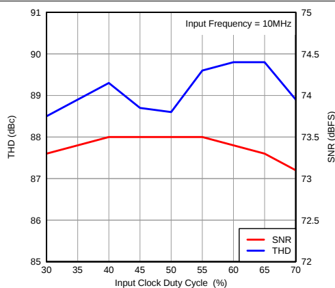
Figure 67. Performance Across Input Clock Duty Cycle
