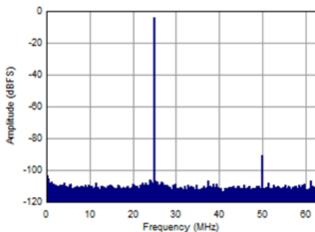
Figure 162. FFT for 100-MHz Input Signal
