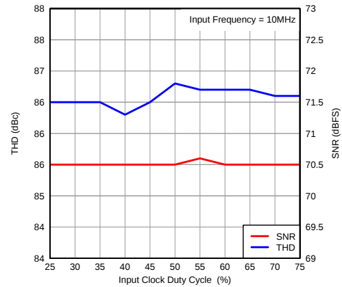
Figure 87. Performance vs Input Clock Duty Cycle
