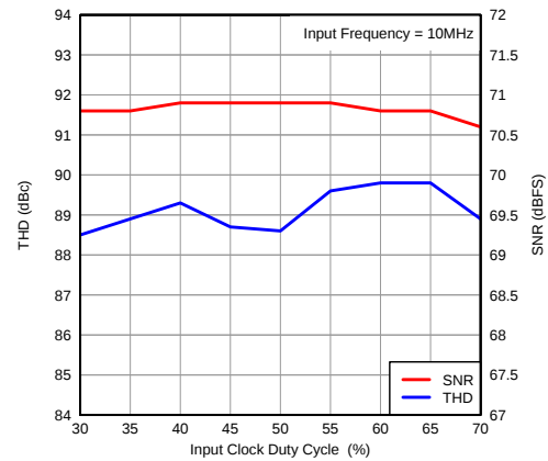
Figure 123. Performance vs Input Clock Duty Cycle
