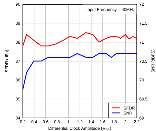
Figure 101. Performance vs Input Clock Amplitude
