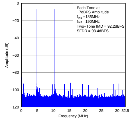
Figure 51. FFT for Two-Tone Input Signal
