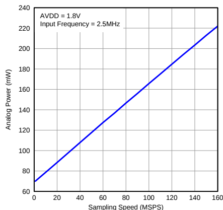
Figure 126. Analog Power vs Sampling Frequency
