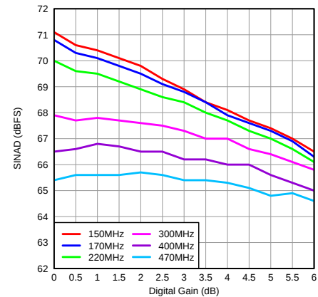
Figure 15. SINAD vs Gain and Input Frequency
