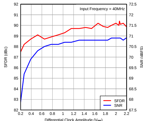
Figure 121. Performance vs Input Clock Amplitude
