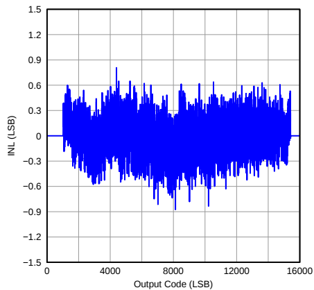
Figure 68. Integrated Nonlinearity
