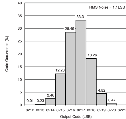
Figure 47. Output Noise Histogram (With Inputs Shorted to VCM)
