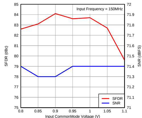
Figure 61. Performance vs Input Common-Mode Voltage
