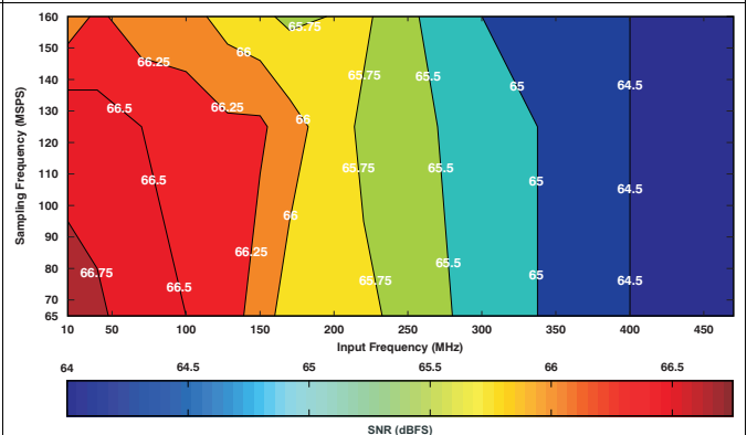
Figure 134. ADS422x Signal-to-Noise Ratio (6-dB Gain)
