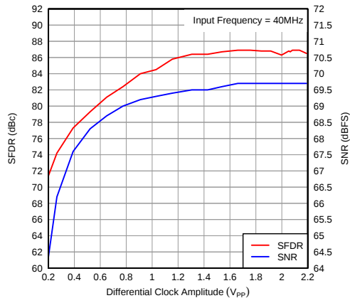
Figure 102. Performance vs Input Clock Amplitude
