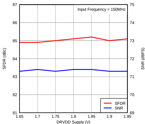
Figure 64. Performance vs DRVDD Supply Voltage
