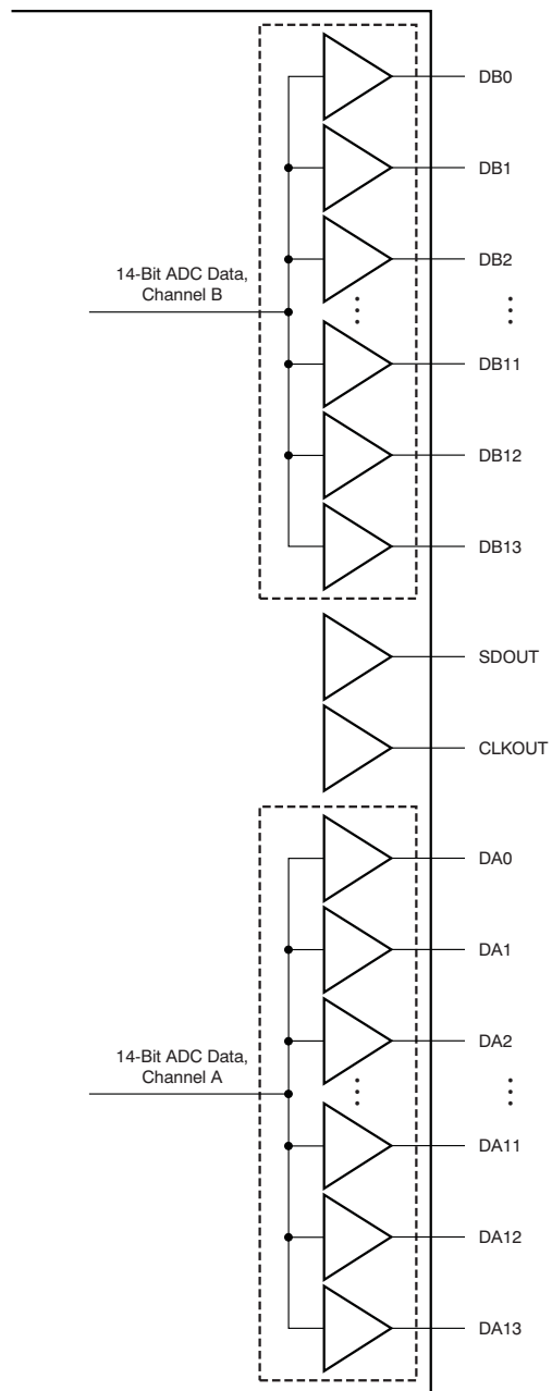
Figure 158. CMOS Outputs
