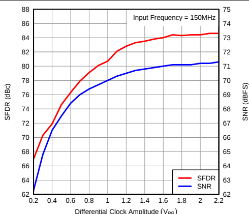
Figure 66. Performance vs Input Clock Amplitude
