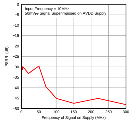
Figure 125. PSRR vs Test Signal Frequency
