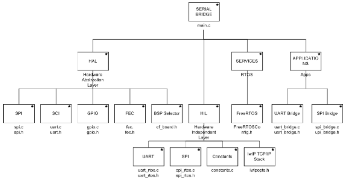
Figure 21. File Implementation
