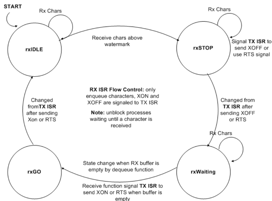
Figure 25. Rx ISR Flow Control State Machine
