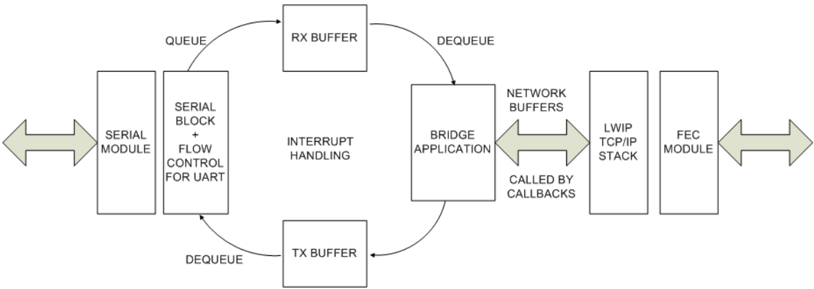
Figure 28. Interrupt Handling
