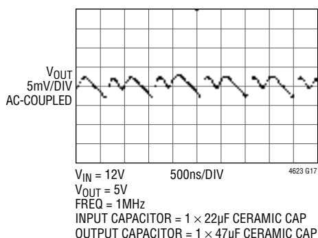
Output Ripple
