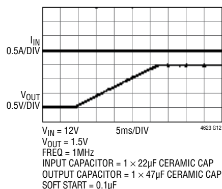
Start-Up with No Load Applied
