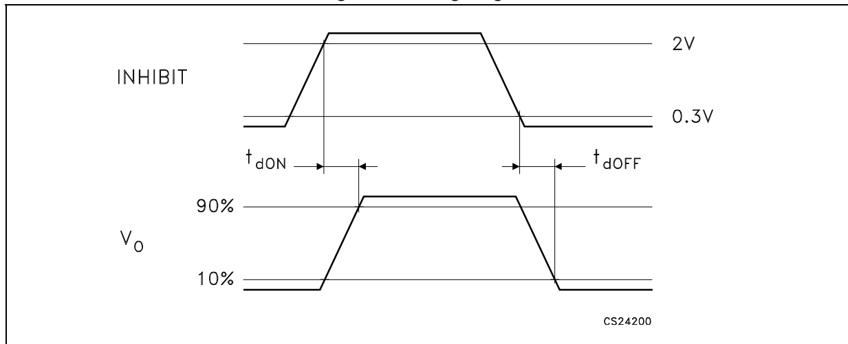
Figure 4. Timing diagram
