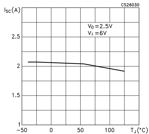
Figure 12. Short-circuit current vs temperature
