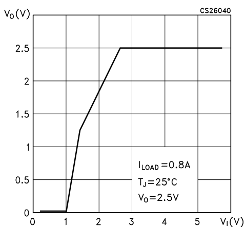
Figure 13. Output voltage vs input voltage
