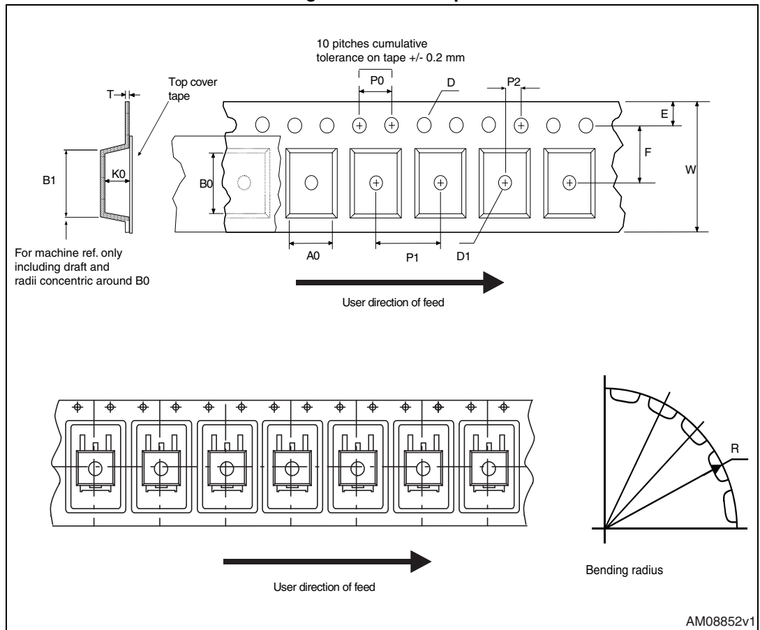
Figure 20. PPAK tape
