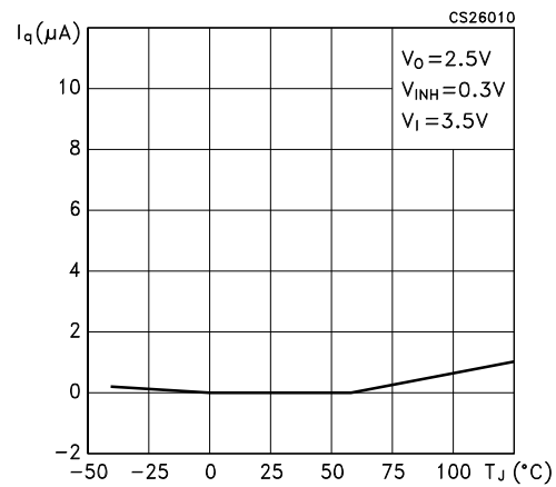
Figure 10. Off-state current vs temperature
