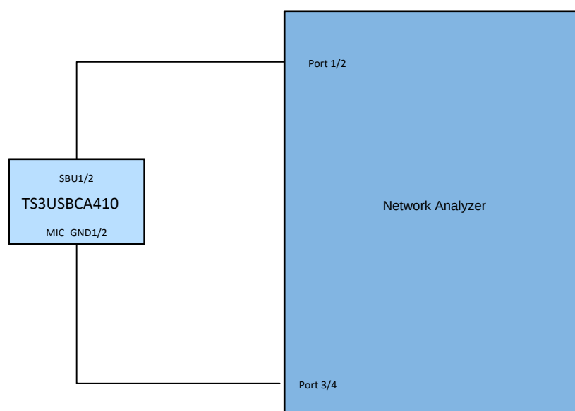
Figure 2. Example Test Board Setup
