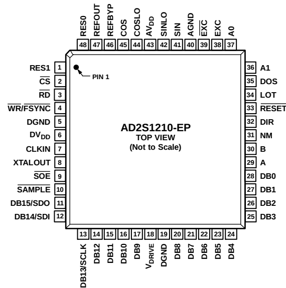
Figure 2. Pin Configuration
