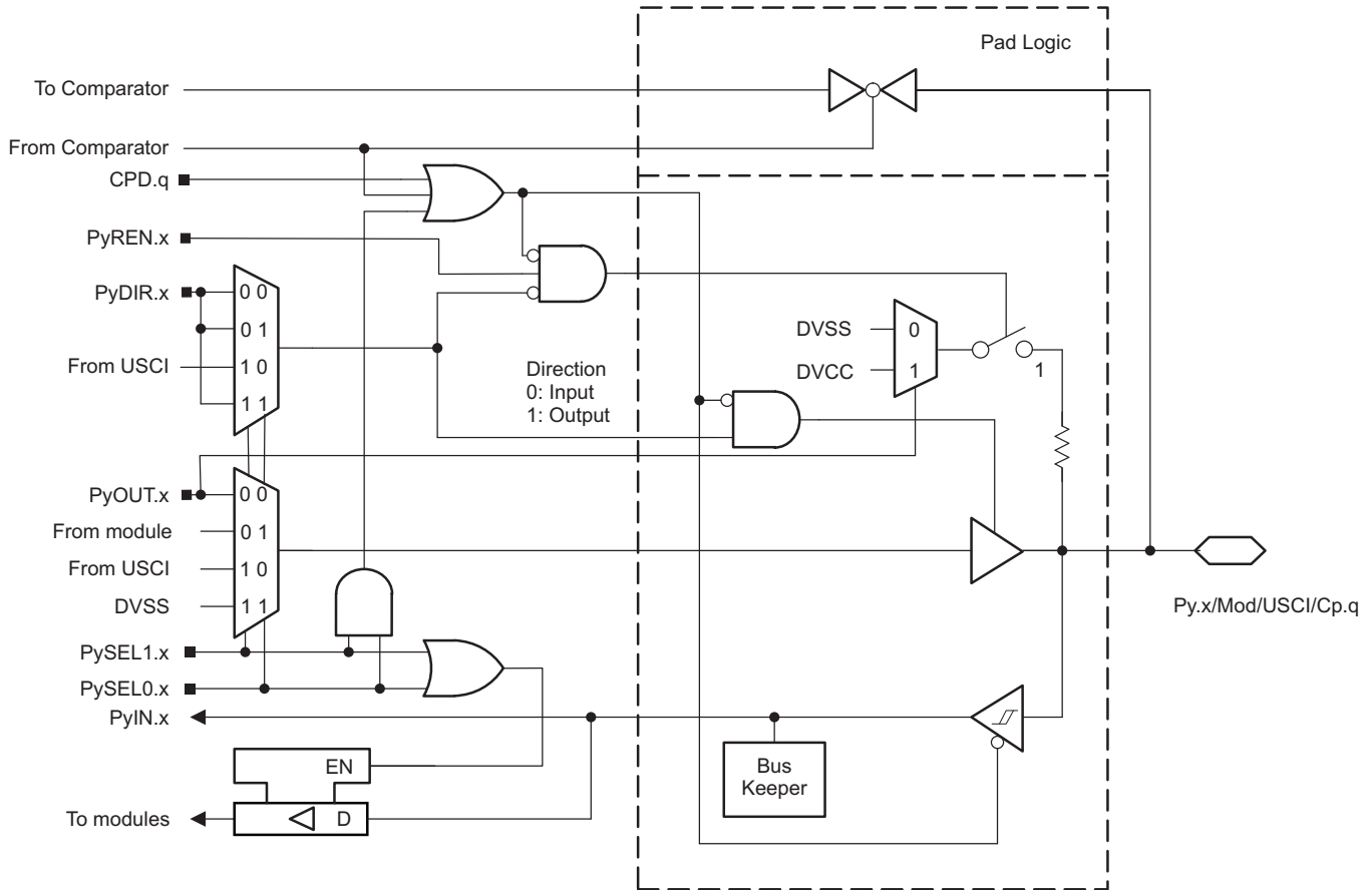
Figure 6-16. Py.x/Mod/USCI/Cp.q Port Schematic
