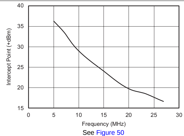
Figure 41. Two-Tone, 3rd-Order Intermodulation Intercept
