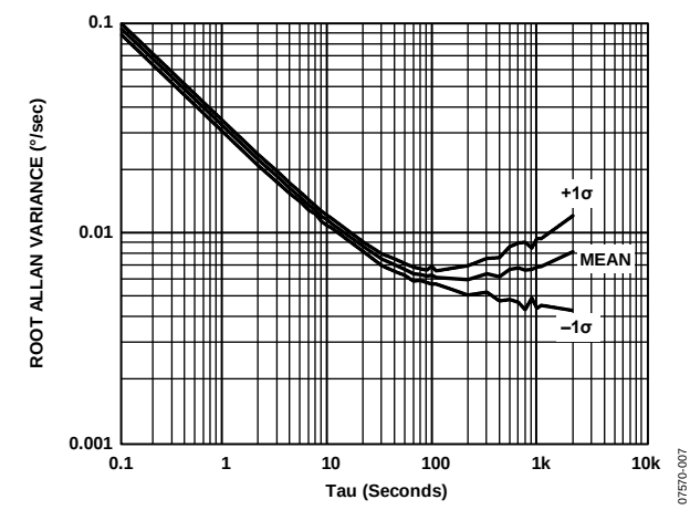
Figure 7. Gyroscope Allan Variance
