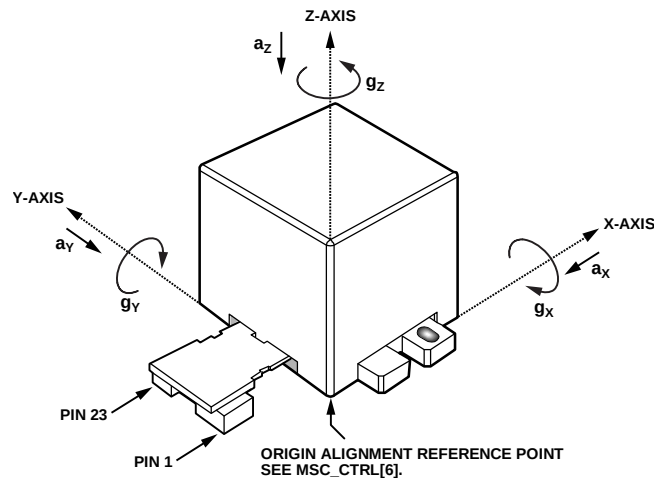
Figure 5. Pin Configuration
