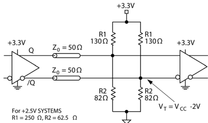
Figure 4. Parallel Termination
