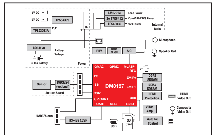
▲ DM8127 IP camera reference design block diagram: TMDXIPCAM8127J3
