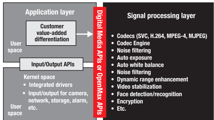
▲ TMS320DMxx-based IP Camera reference design software
