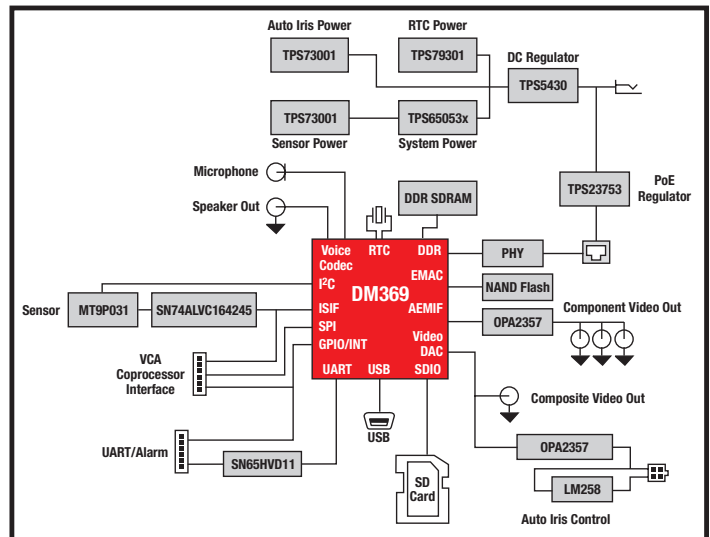
▲ IP camera reference design block diagram: TMSIPCAM369X104
