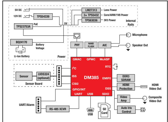
▲ DM385 IP camera reference design block diagram: TMSIPCAM385M34
