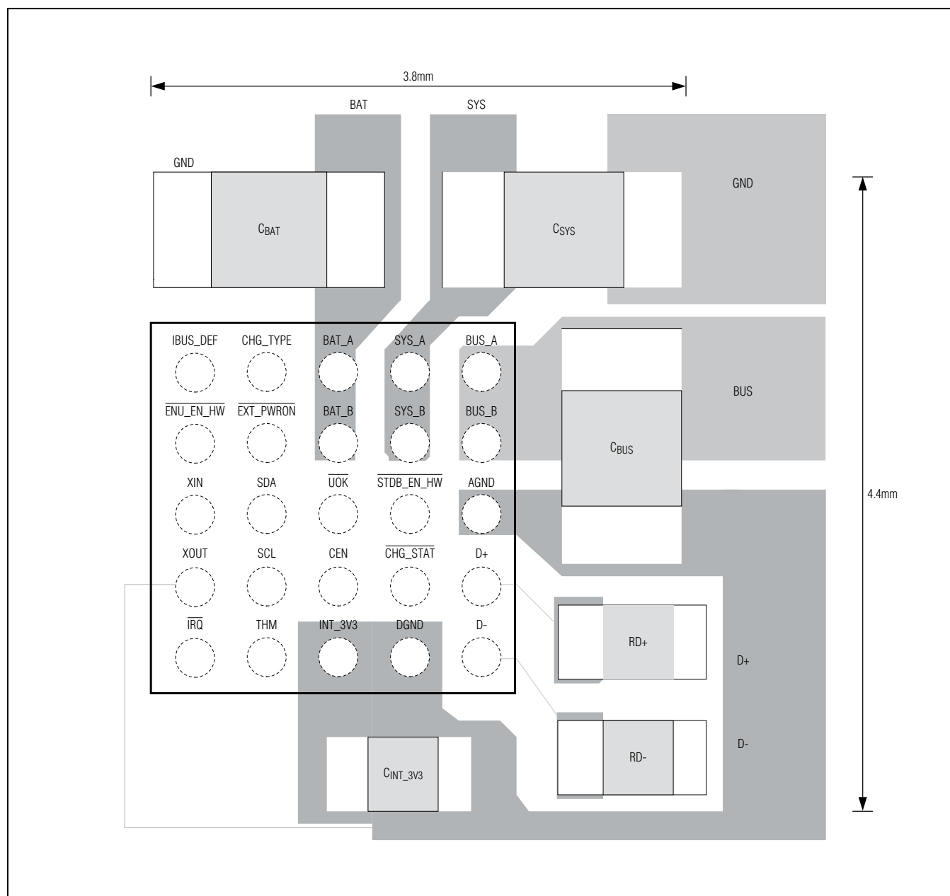
Figure 26. Recommended PCB Layout for Low Speed
