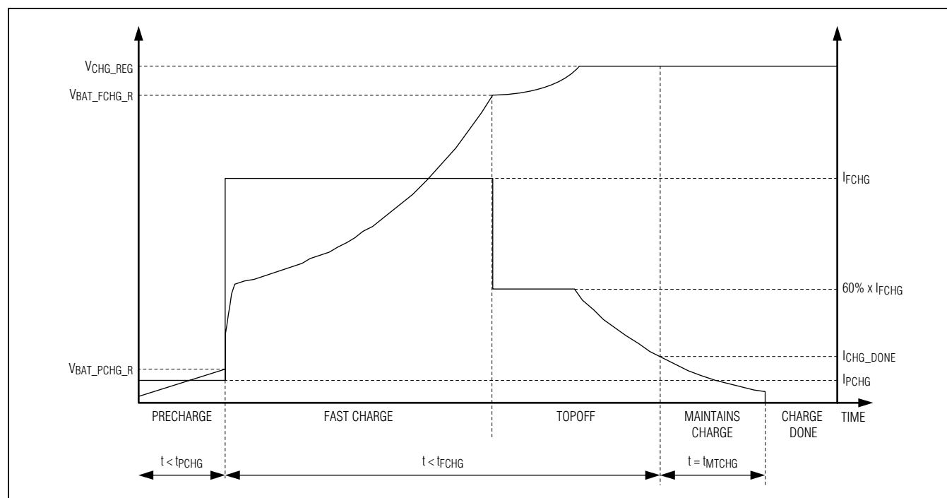
Figure 10. Charge Profile
