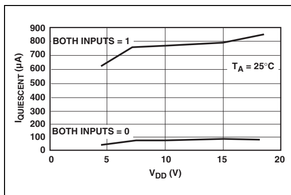
FIGURE 2-14: Quiescent Supply Current vs. Voltage.
