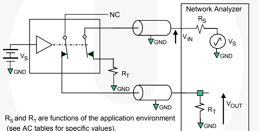
Figure 13. Channel-to-Channel Crosstalk
