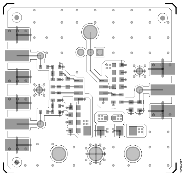
Figure 7. EVAL-LTC6228IS8E Layout Pattern, Primary Side
