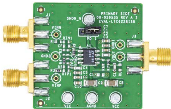
Figure 1. EVAL-LTC6228IS8, Primary Side
