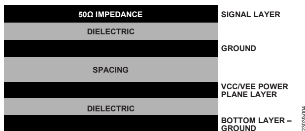
Figure 4. Stack Up
