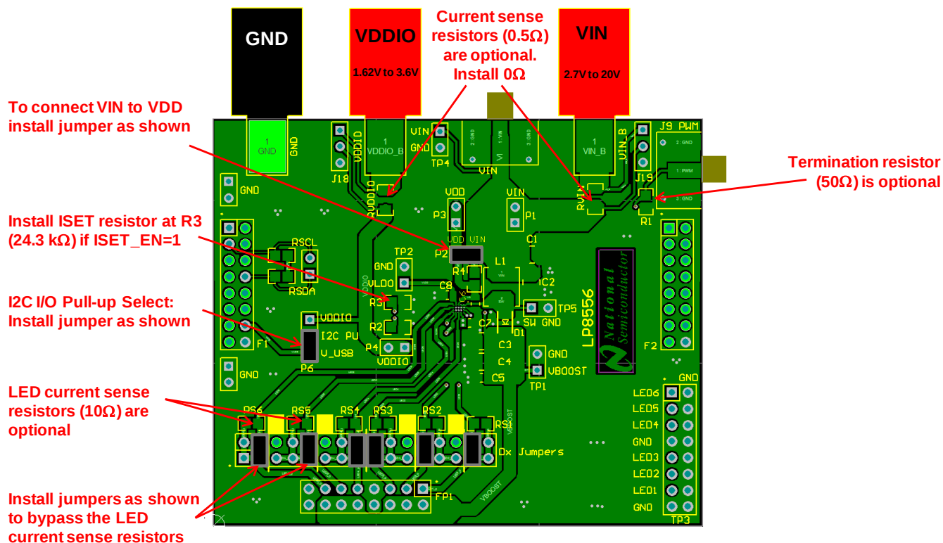
Figure 3: LP8556TM-EVM Configuration
