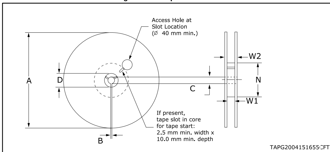
Figure 39: Octapak reel 13"
