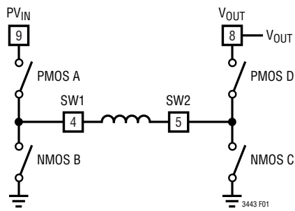
Figure 1. Simplified Diagram of Output Switches
