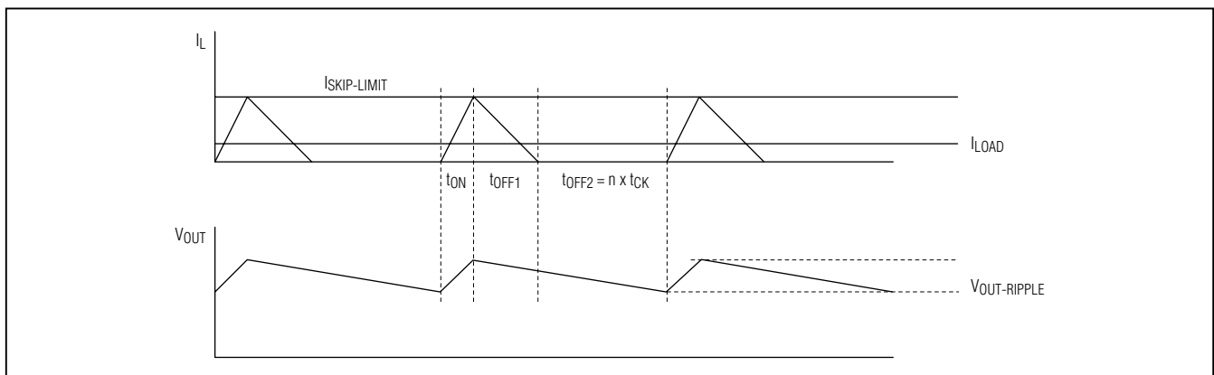
Figure 3. Skip-Mode Waveforms
