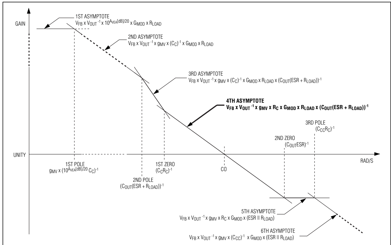
Figure 4. Asymptotic Loop Response of Peak Current-Mode Regulator
