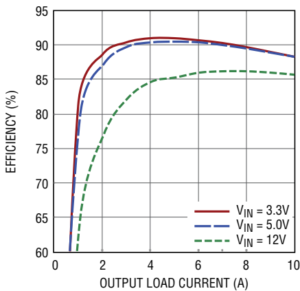
Efficiency vs Load Current at V_O = 1.8V , f_{SW} = 500kHz
