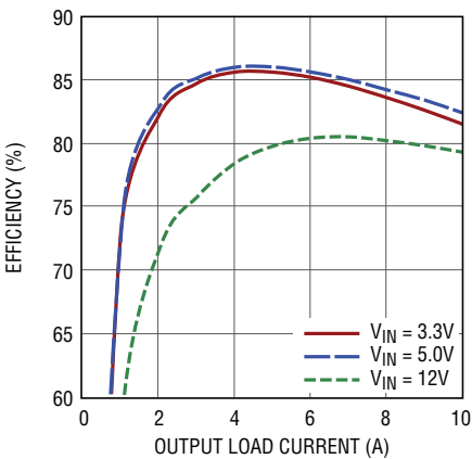
Efficiency vs Load Current at V_O = 1.0V , f_{SW} = 500kHz
