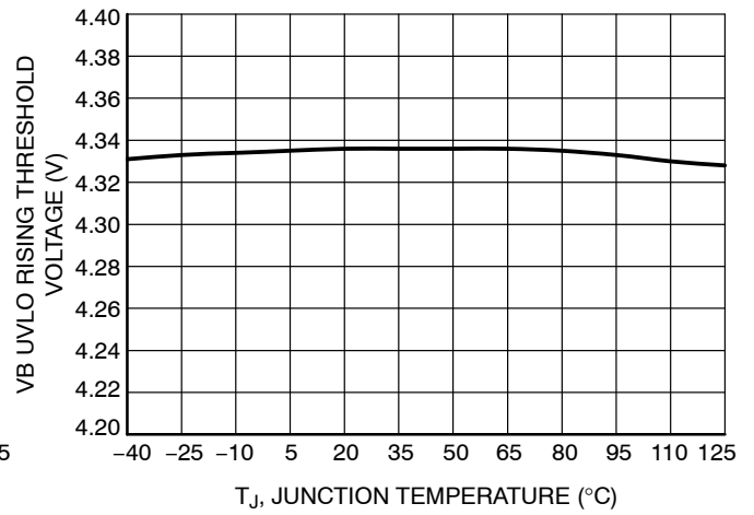
Figure 13. VB UVLO Rising Threshold vs. Junction Temperature
