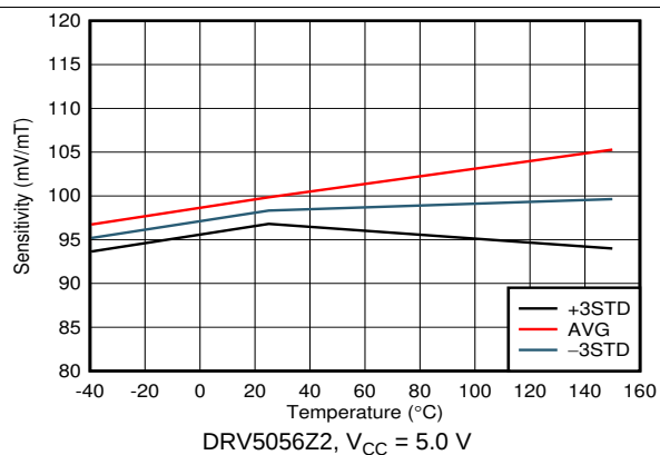
Figure 22. Sensitivity vs Temperature
