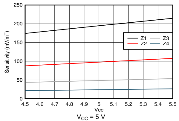
Figure 18. Sensitivity vs Supply Voltage
