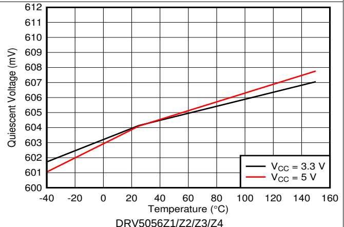
Figure 16. Quiescent Voltage vs Temperature
