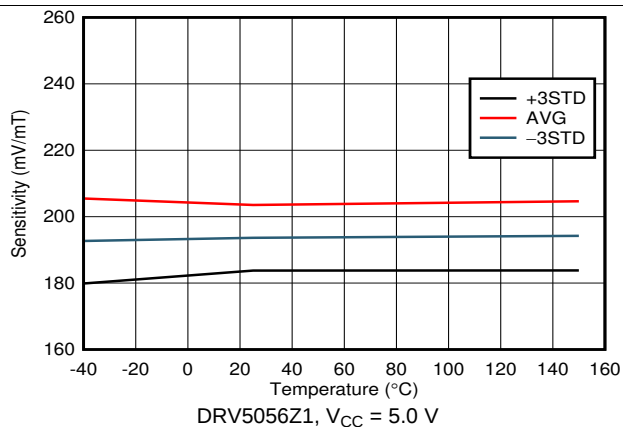
Figure 20. Sensitivity vs Temperature
