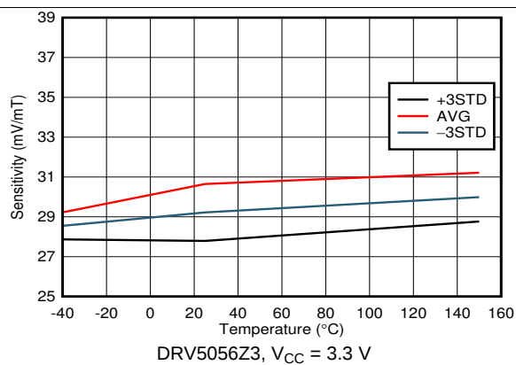
Figure 23. Sensitivity vs Temperature
