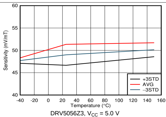
Figure 24. Sensitivity vs Temperature
