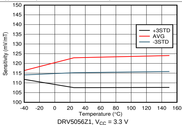
Figure 19. Sensitivity vs Temperature
