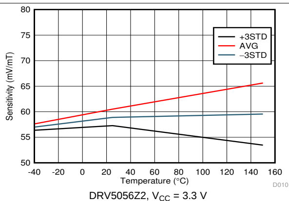
Figure 21. Sensitivity vs Temperature
