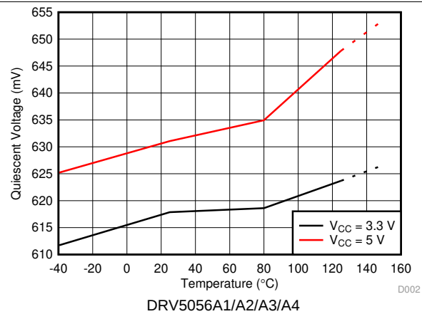
Figure 3. Quiescent Voltage vs Temperature
