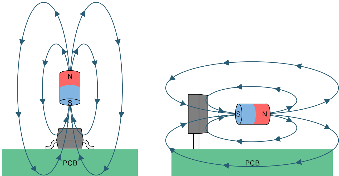
Figure 28. The Flux Direction for Positive B
