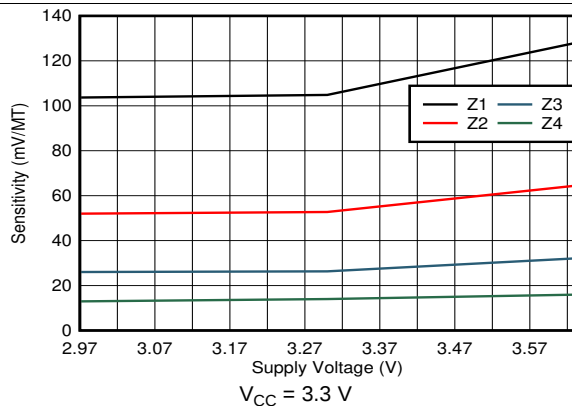
Figure 17. Sensitivity vs Supply Voltage
