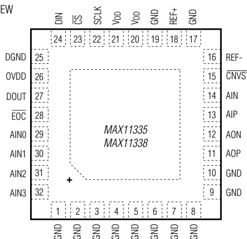
TQFN 4 CHANNEL
