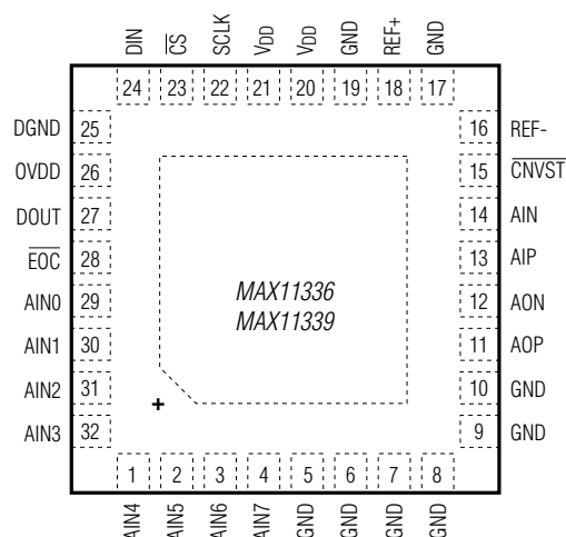
TQFN 8 CHANNEL
