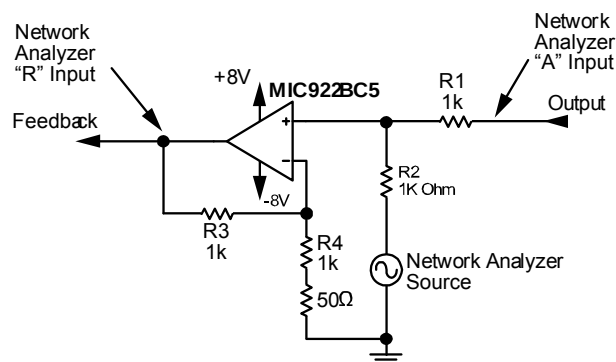
Figure 8. Op Amp Injection
