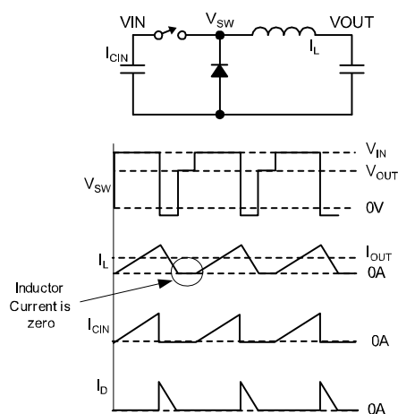
Figure 5. Discontinuous Operation
