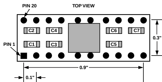
Figure 2. EVAL-ADXRS622 Parts Layout
