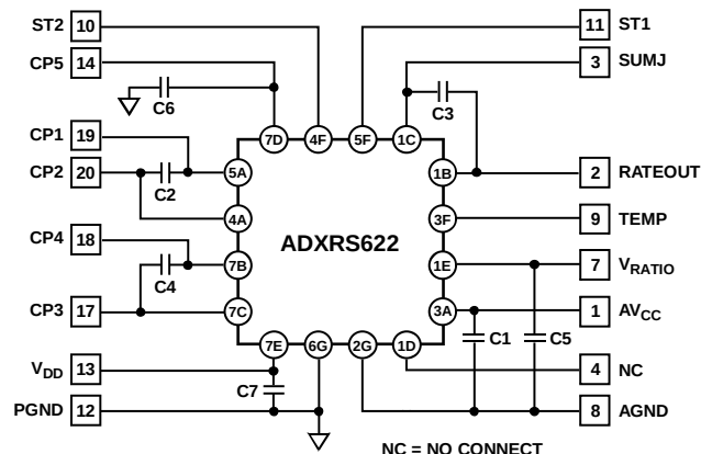
Figure 1. EVAL-ADXRS622 Schematic
