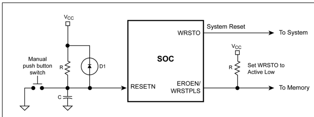
FIGURE 2-13: RESET CIRCUIT
