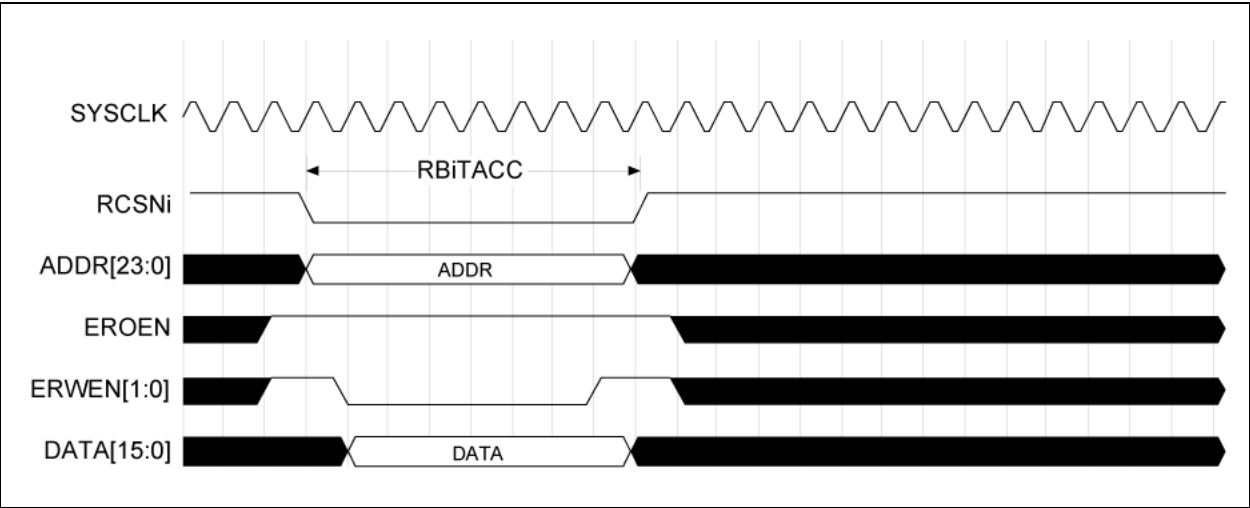
FIGURE 5-3: STATIC MEMORY WRITE CYCLE
