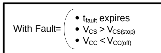
Figure 53. Controller Operation State Diagram (Latched Protection)
