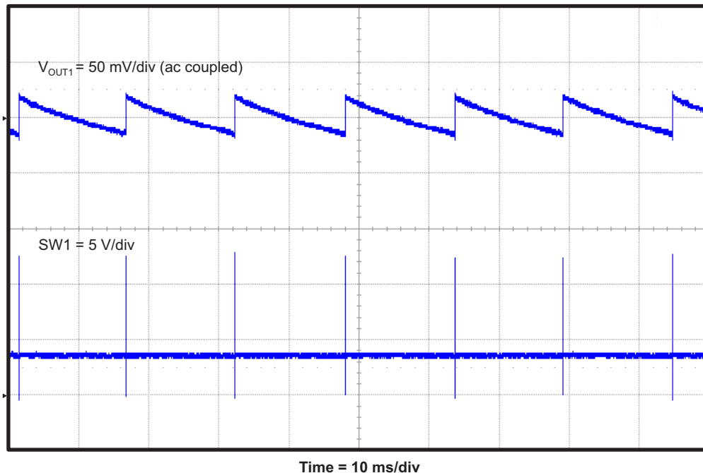
Figure 12. TPS542951EVM Converter 1 Eco-mode™ Output Voltage Ripple at No Load
