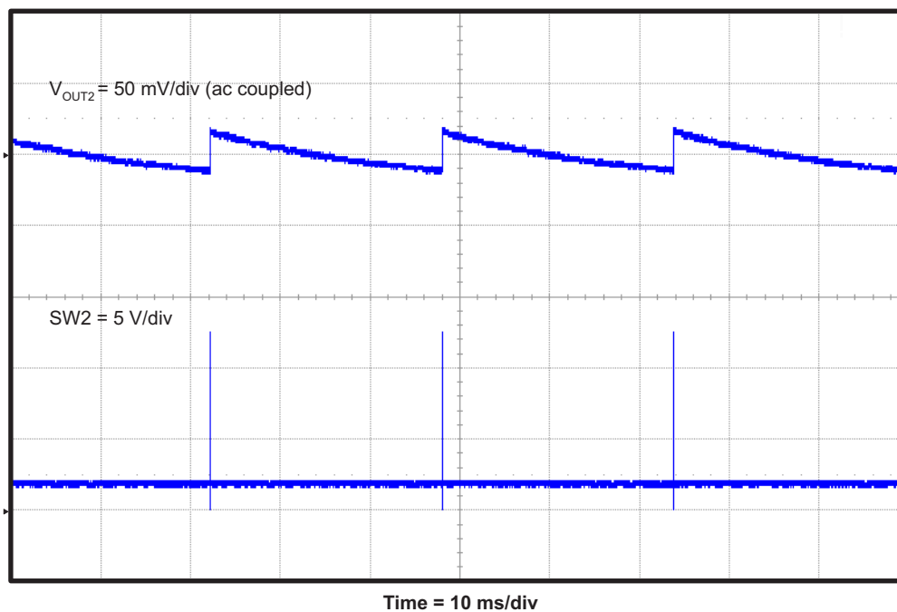
Figure 14. TPS542951EVM Converter 2 Eco-mode™ Output Voltage Ripple at No Load
