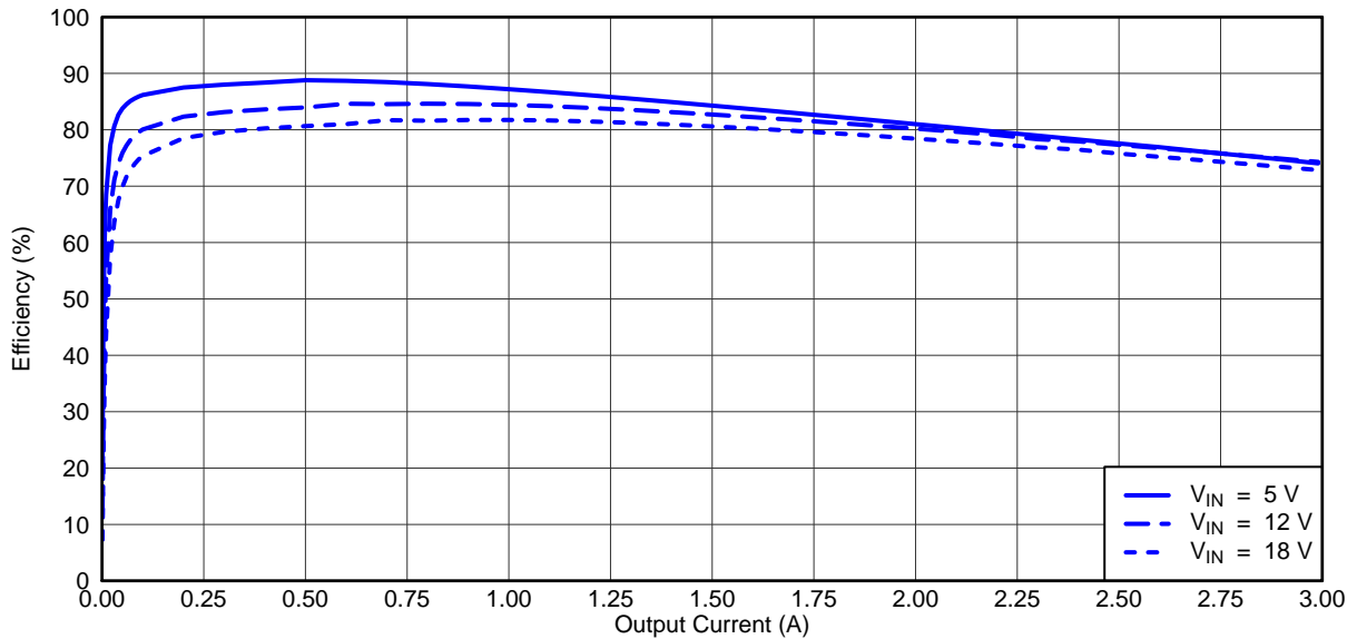
Figure 3. TPS542951EVM Converter 2 Efficiency
