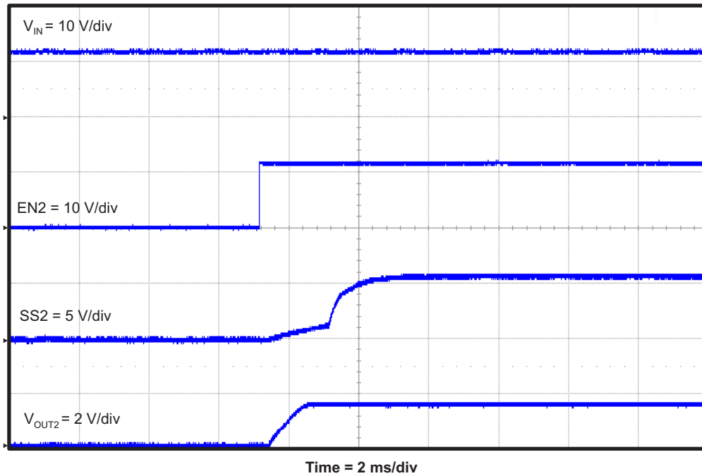
Figure 19. TPS542951EVM Start-Up Relative to EN2
