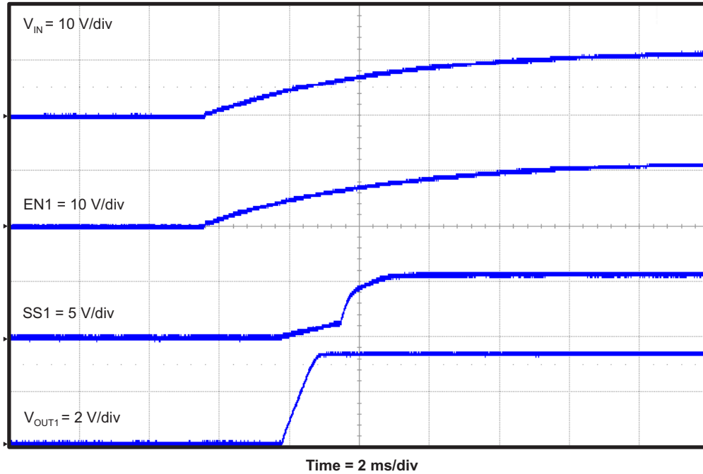
Figure 16. TPS542951EVM Converter 1 Start-Up Relative to V_{IN}
