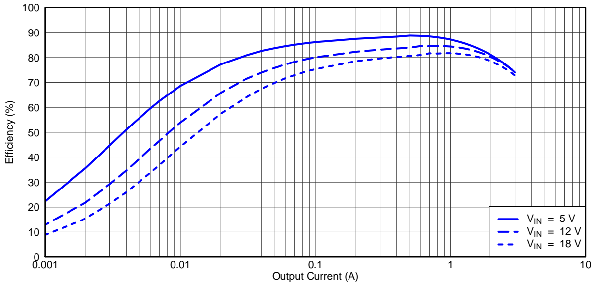
Figure 4. TPS542951EVM Converter 2 Light Load Efficiency
