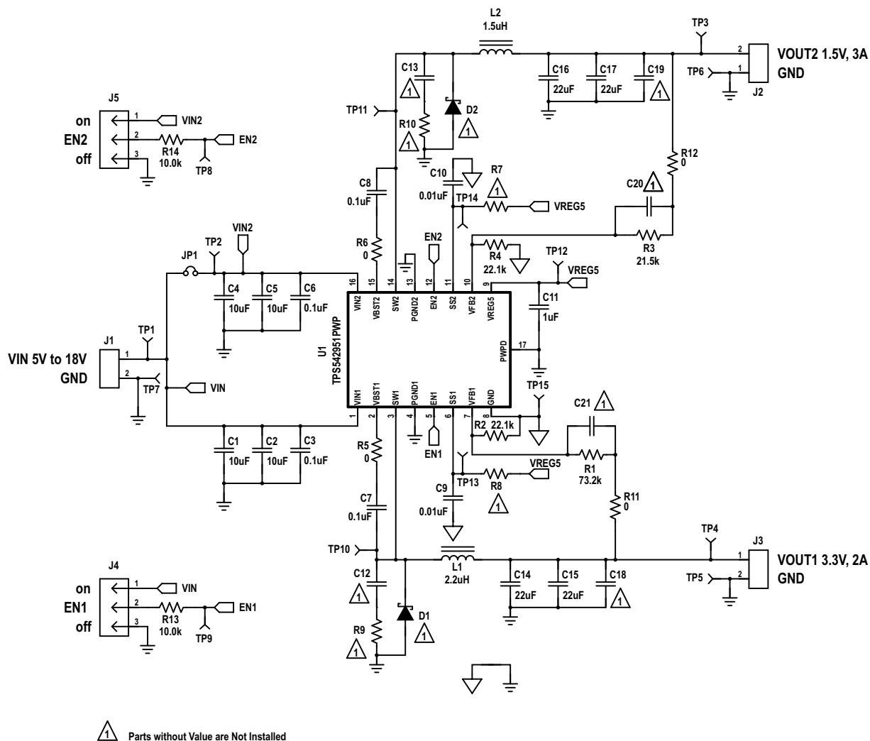
Figure 26. TPS542951EVM Schematic Diagram
