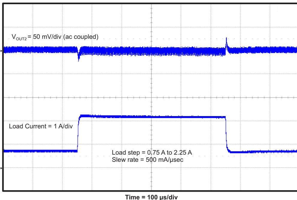
Figure 10. TPS542951EVM Converter 2 Load Transient Response
