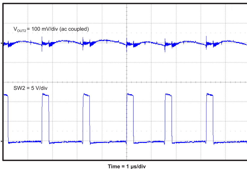
Figure 13. TPS542951EVM Converter 2 Output Voltage Ripple
