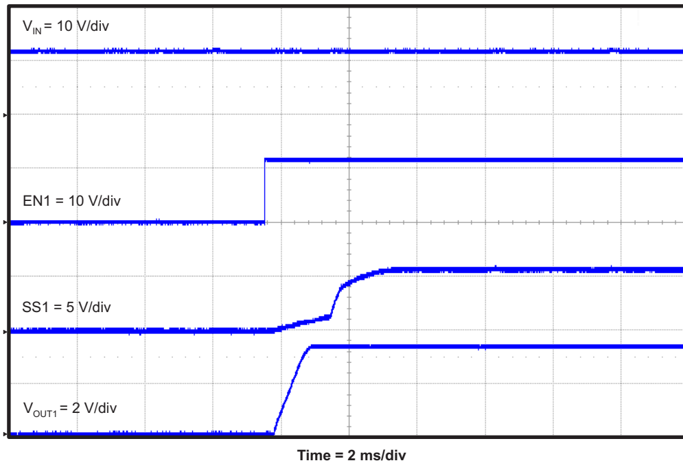
Figure 17. TPS542951EVM Start-Up Relative to EN1
