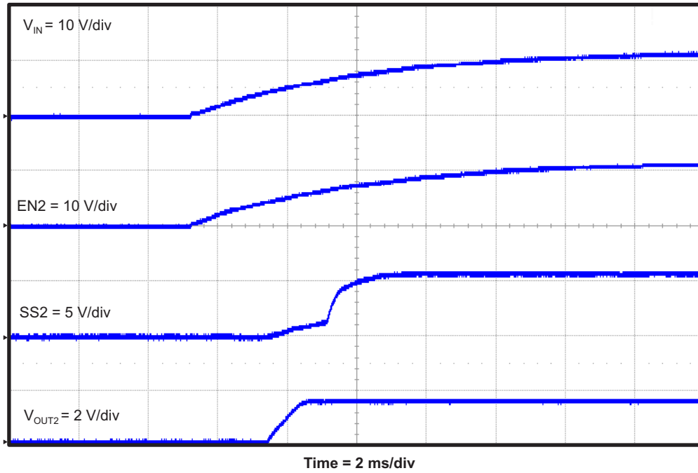
Figure 18. TPS542951EVM Converter 2 Start-Up Relative to V_{IN}
