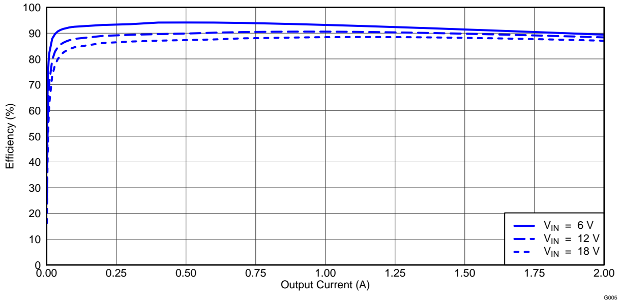
Figure 1. TPS542951EVM Converter 1 Efficiency
