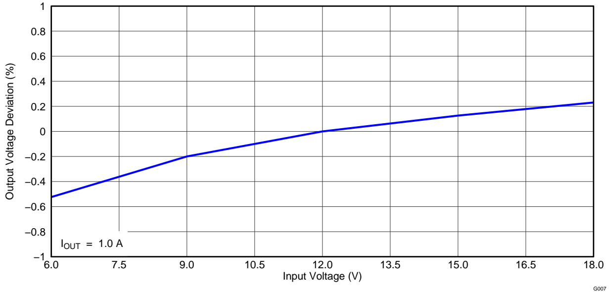
Figure 7. TPS542951EVM Converter 1 Line Regulation
