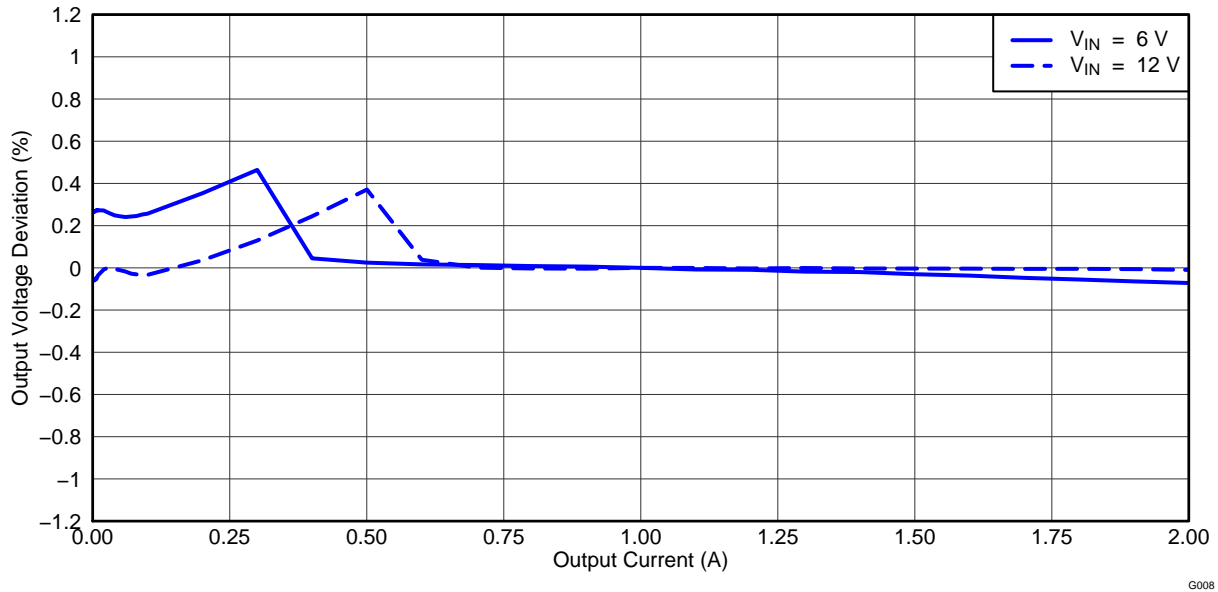
Figure 5. TPS542951EVM Converter 1 Load Regulation
