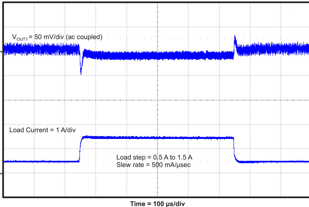
Figure 9. TPS542951EVM Converter 1 Load Transient Response
