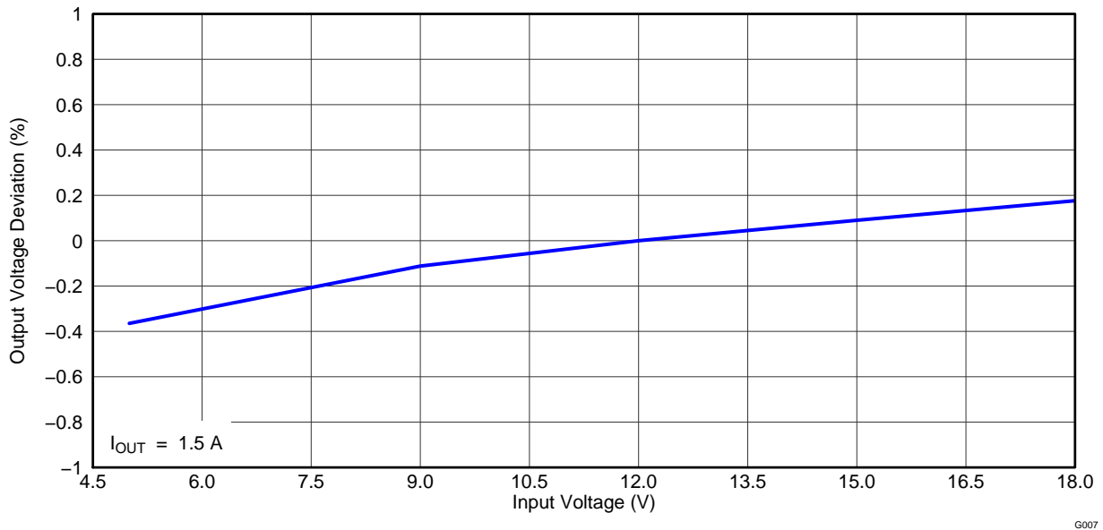
Figure 8. TPS542951EVM Converter 2 Line Regulation
