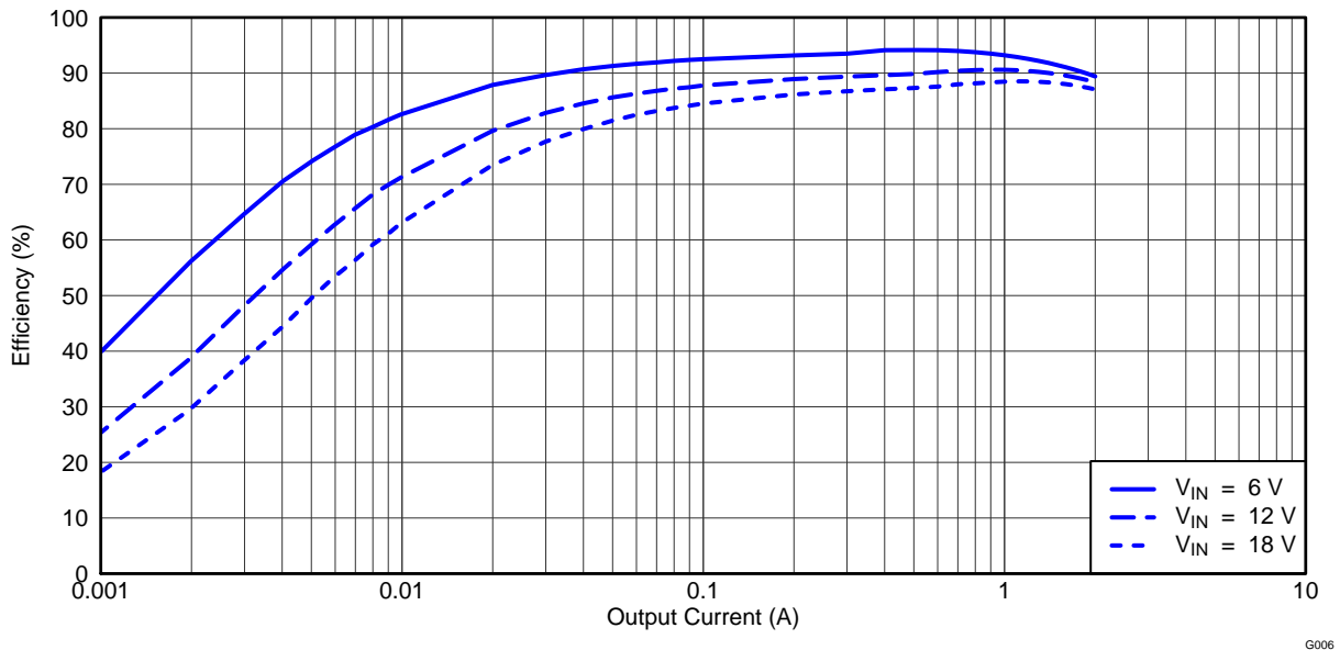
Figure 2. TPS542951EVM Converter 1 Light Load Efficiency
