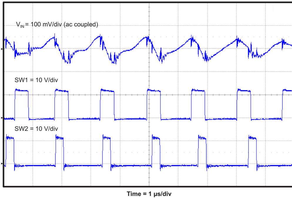
Figure 15. TPS542951EVM Input Voltage Ripple
