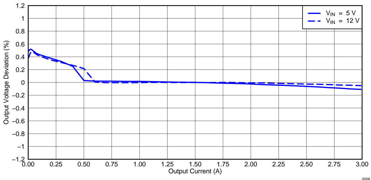
Figure 6. TPS542951EVM Converter 2 Load Regulation
