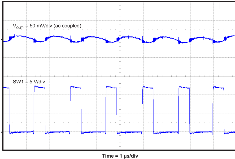
Figure 11. TPS542951EVM Converter 1 Output Voltage Ripple
